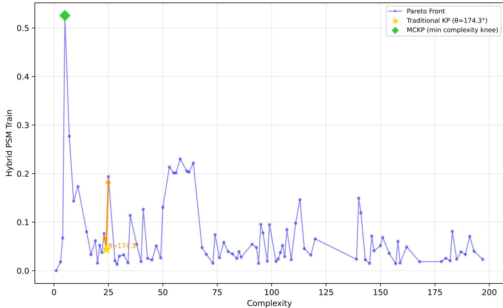
542_pollution - Run 19 - SVP - Hybrid PSM Train \lambda_1=0.00, \lambda_2=0.00, \lambda_3=0.20 | Difficulty: 0.72 | Method: hmr
