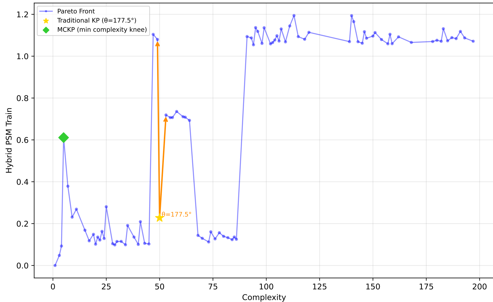
542_pollution - Run 19 - SVP - Hybrid PSM Train \lambda_1=0.70, \lambda_2=1.00, \lambda_3=0.10 | Difficulty: 0.72 | Method: hmr
