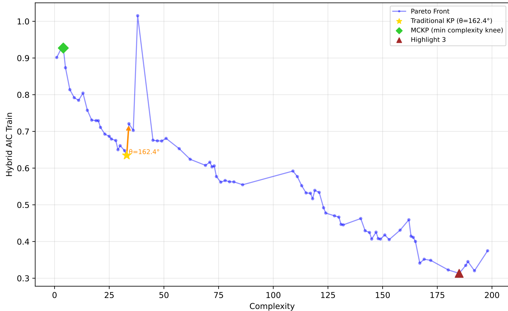
542_pollution - Run 1 - MVP - Hybrid AIC Train \lambda_1=0.40, \lambda_2=0.10, \lambda_3=0.00 | Difficulty: 0.95 | Method: hmr
