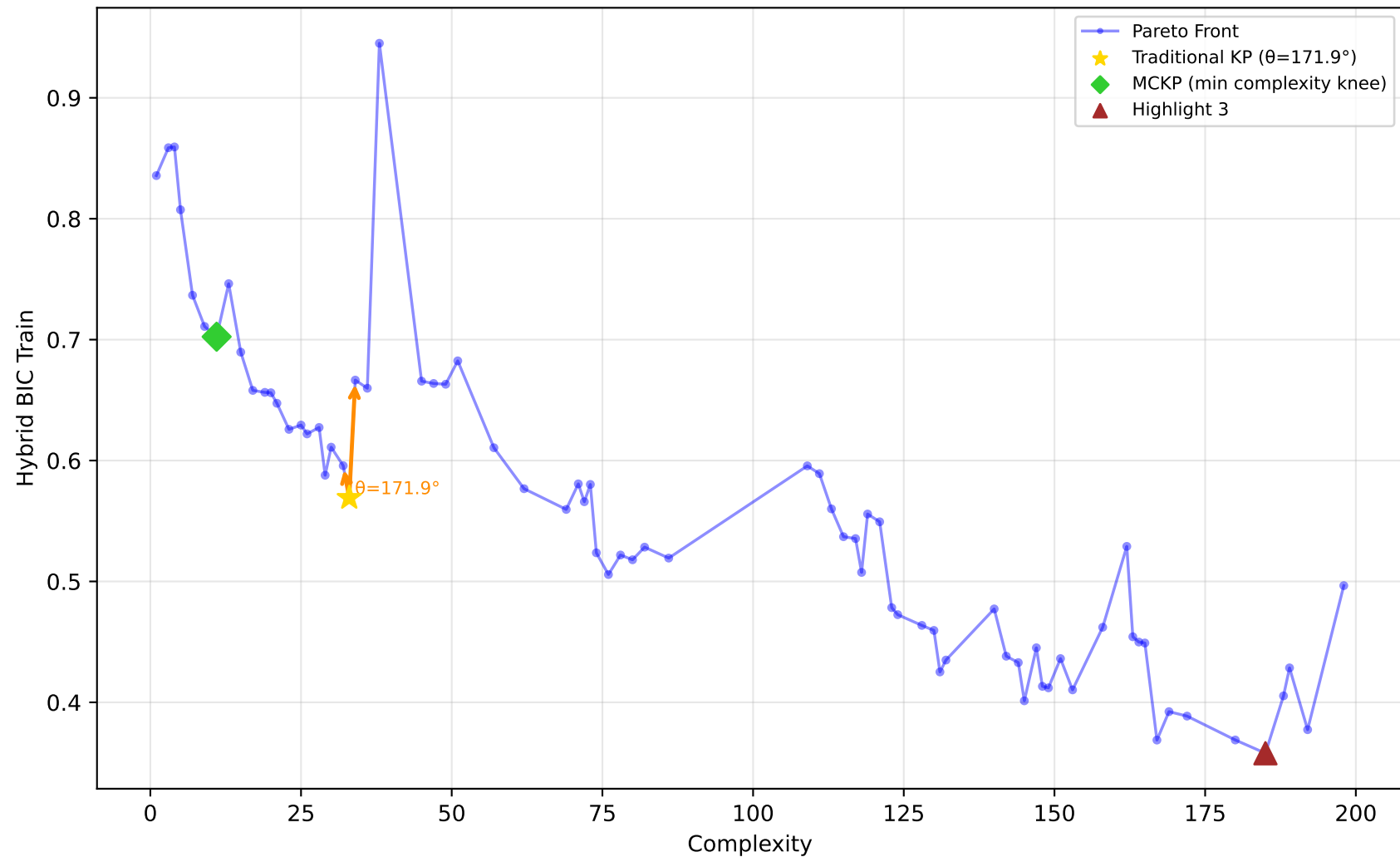
542_pollution - Run 1 - MVP - Hybrid BIC Train \lambda_1=0.40 , \lambda_2=0.10 , \lambda_3=0.00 | Difficulty: 0.95 | Method: hmr
