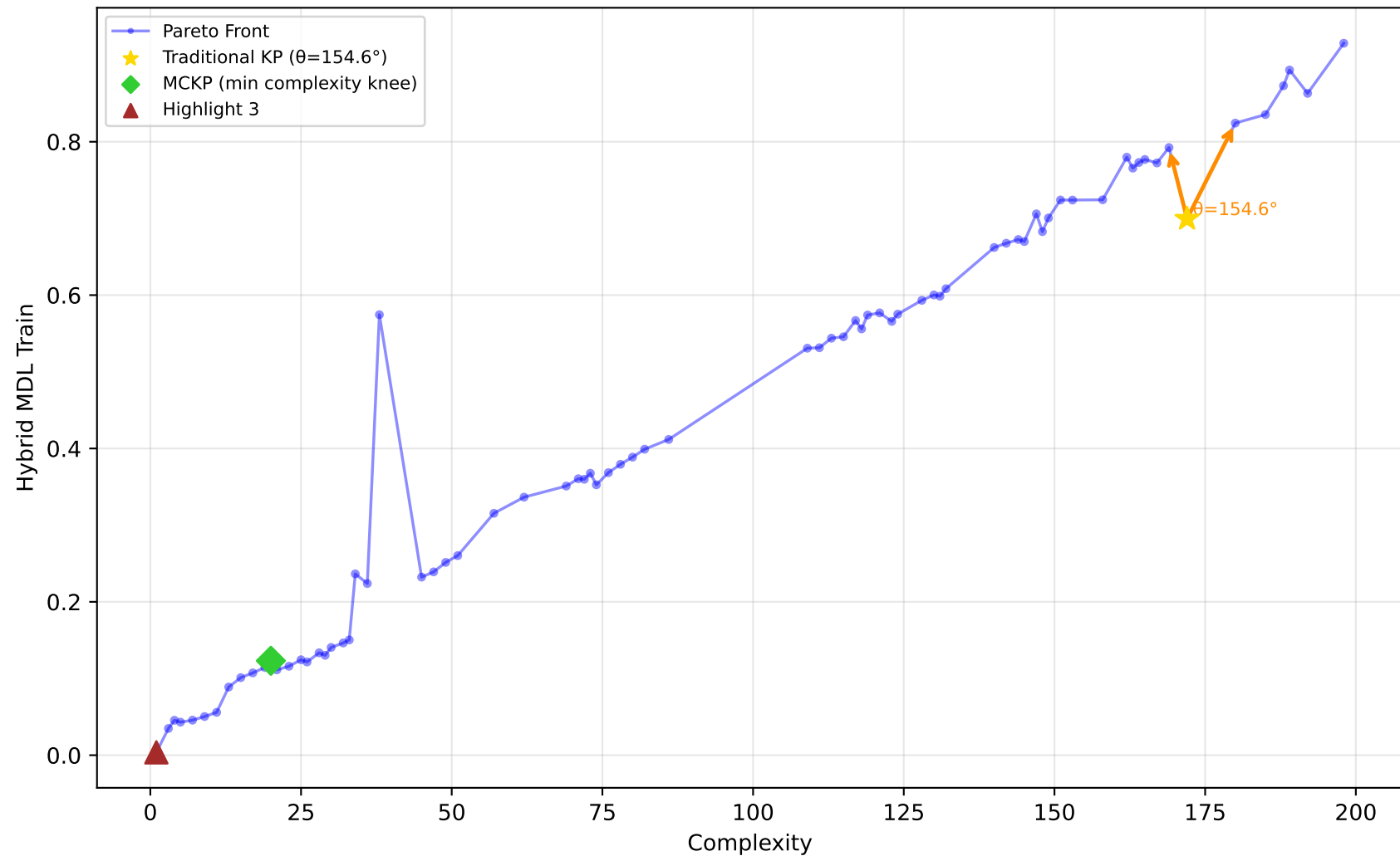
542_pollution - Run 1 - MVP - Hybrid MDL Train \lambda_1=0.40, \lambda_2=0.10, \lambda_3=0.00 | Difficulty: 0.95 | Method: hmr
