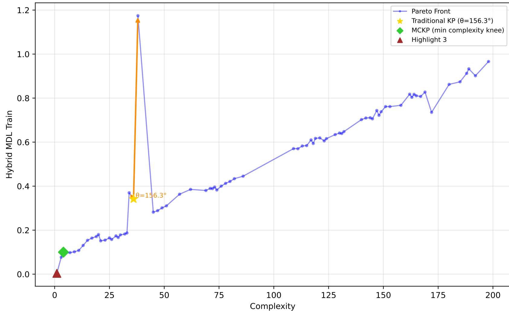
542_pollution - Run 1 - MVP - Hybrid MDL Train \lambda_1=1.00, \lambda_2=0.10, \lambda_3=0.00 | Difficulty: 0.95 | Method: hmr
