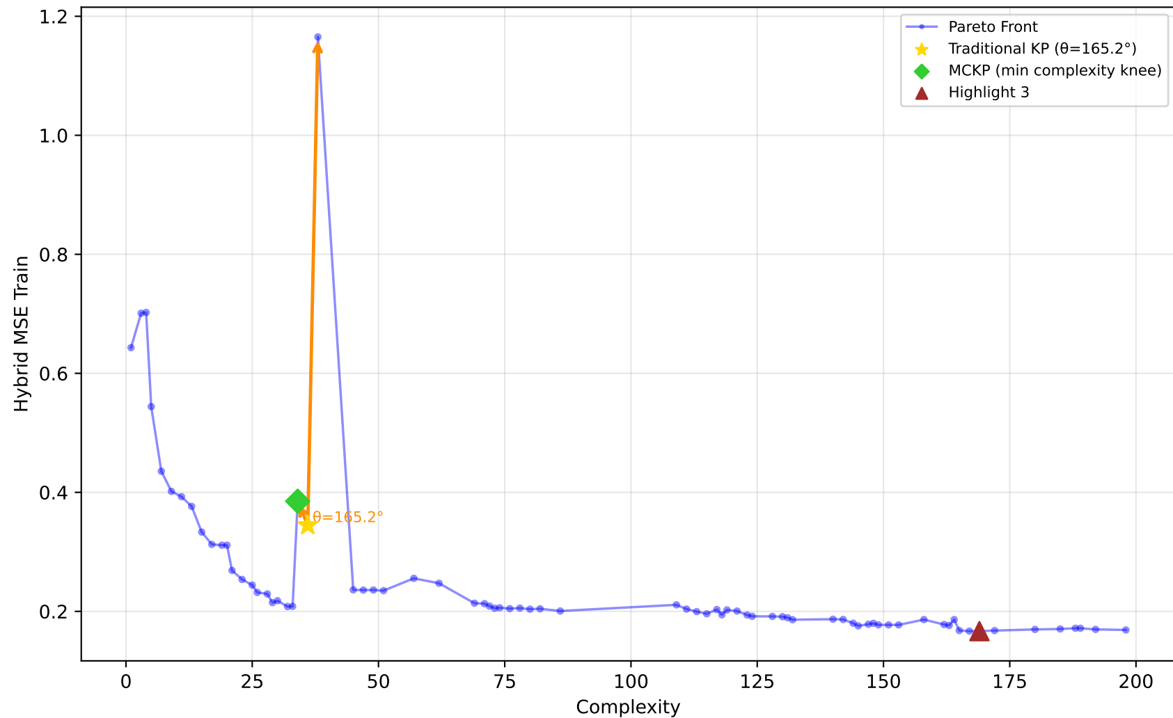
542_pollution - Run 1 - MVP - Hybrid MSE Train \lambda_1=1.00, \lambda_2=0.10, \lambda_3=0.00 | Difficulty: 0.95 | Method: hmr
