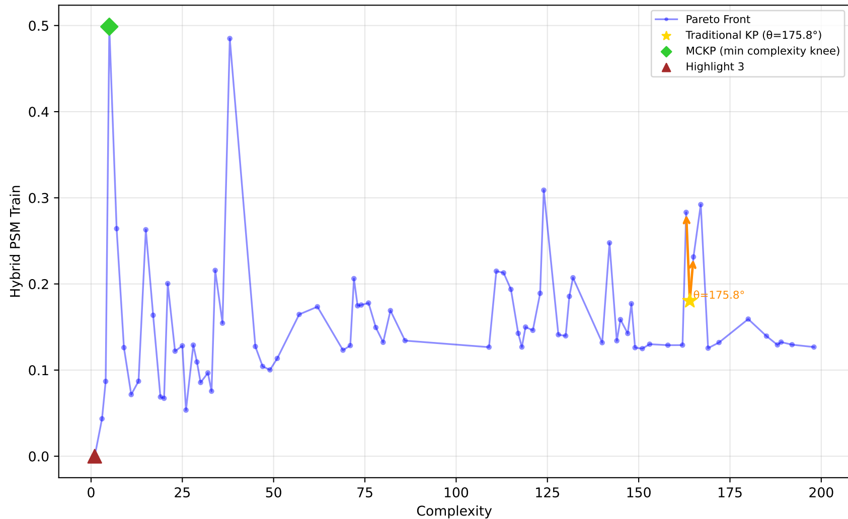
542_pollution - Run 1 - MVP - Hybrid PSM Train \lambda_1=0.40, \lambda_2=0.10, \lambda_3=0.00 | Difficulty: 0.95 | Method: hmr
