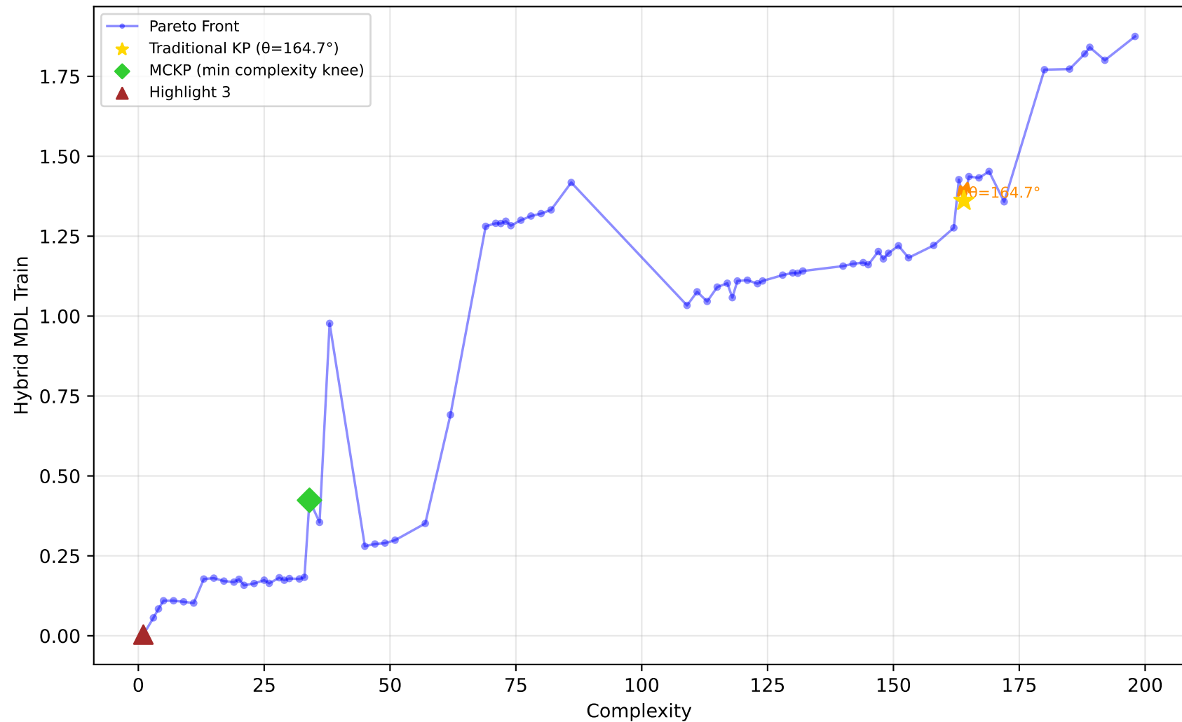
542_pollution - Run 1 - SVP - Hybrid MDL Train \lambda_1=0.70 , \lambda_2=1.00 , \lambda_3=0.10 | Difficulty: 0.95 | Method: hmr
