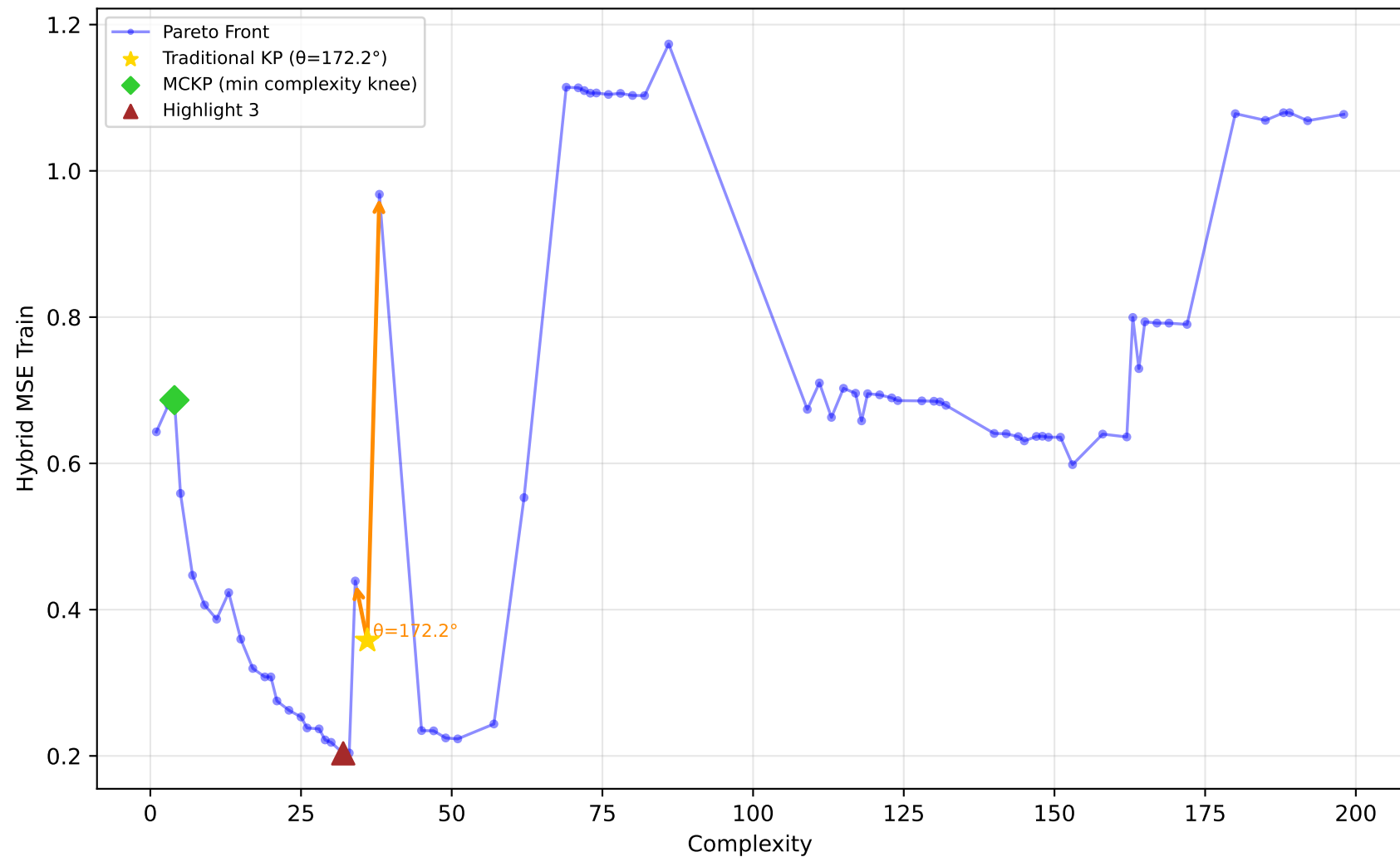
542_pollution - Run 1 - SVP - Hybrid MSE Train \lambda_1=0.70, \lambda_2=1.00, \lambda_3=0.10 | Difficulty: 0.95 | Method: hmr
