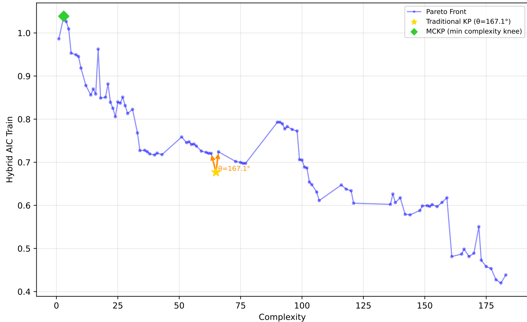
542_pollution - Run 20 - MVP - Hybrid AIC Train \lambda_1=1.00, \lambda_2=0.10, \lambda_3=0.00 | Difficulty: 0.63 | Method: hmr
