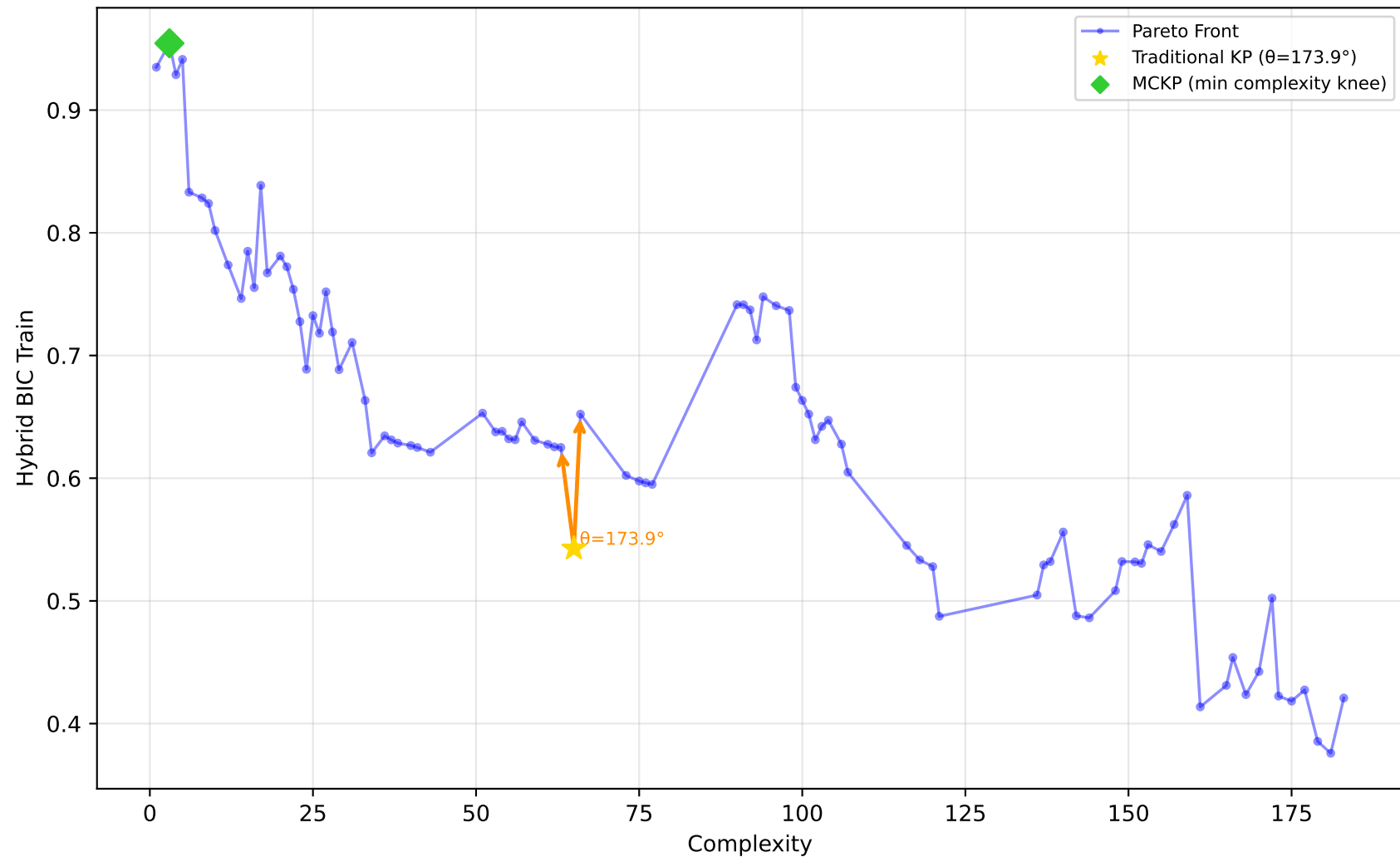
542_pollution - Run 20 - MVP - Hybrid BIC Train \lambda_1=0.40, \lambda_2=0.10, \lambda_3=0.00 | Difficulty: 0.63 | Method: hmr
