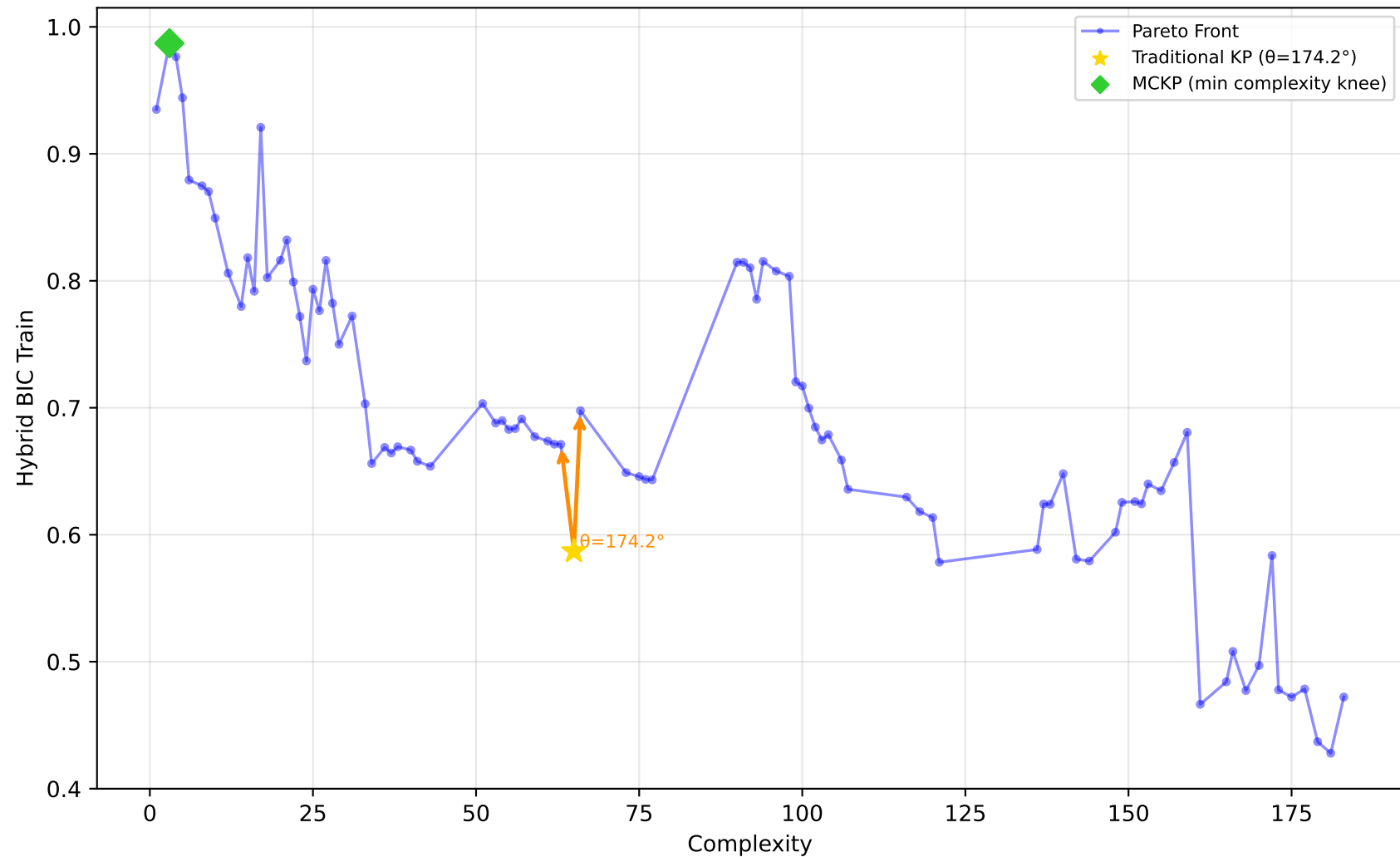
542_pollution - Run 20 - MVP - Hybrid BIC Train \lambda_1=1.00, \lambda_2=0.10, \lambda_3=0.00 | Difficulty: 0.63 | Method: hmr
