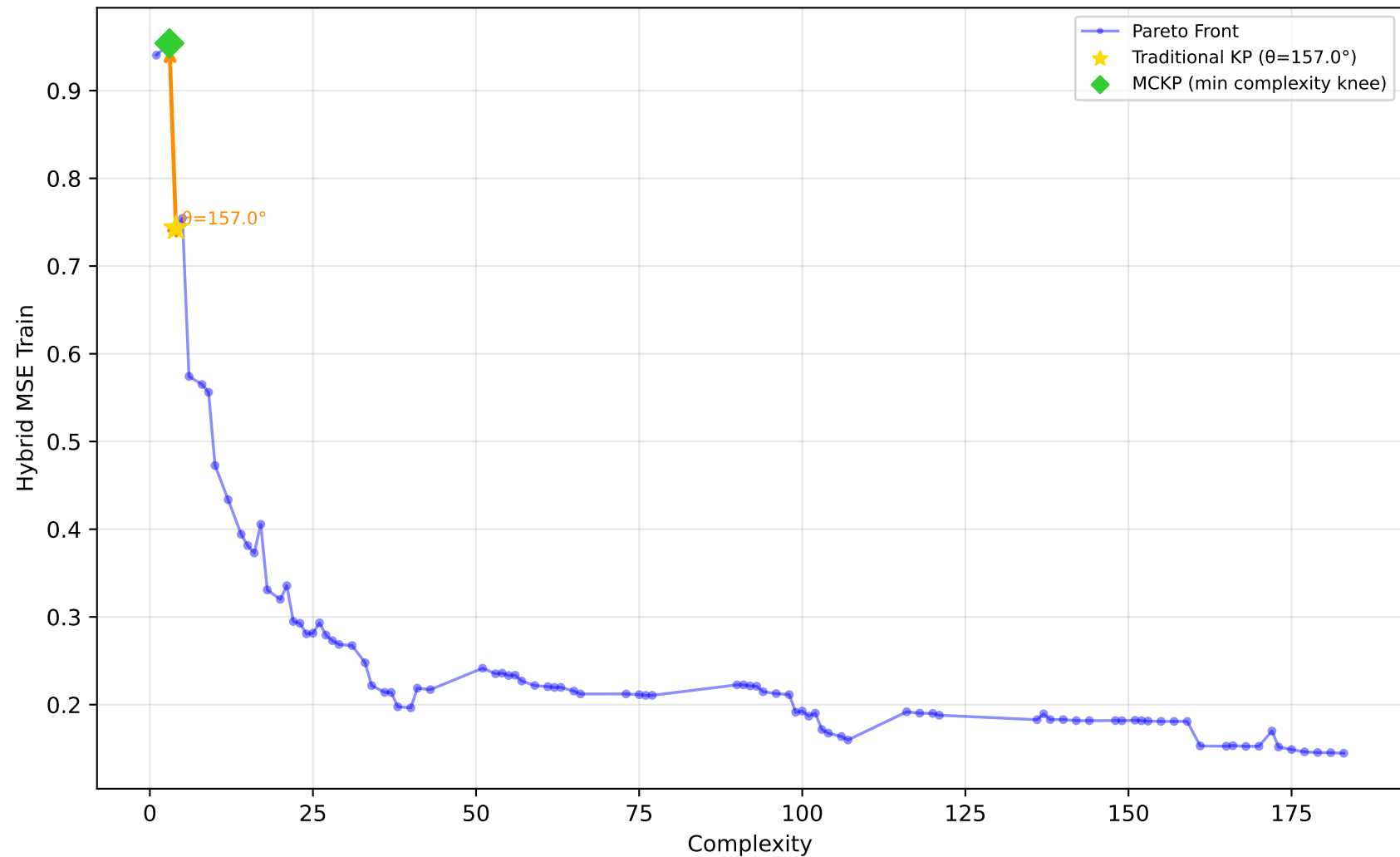
542_pollution - Run 20 - MVP - Hybrid MSE Train \lambda_1=0.40, \lambda_2=0.10, \lambda_3=0.00 | Difficulty: 0.63 | Method: hmr
