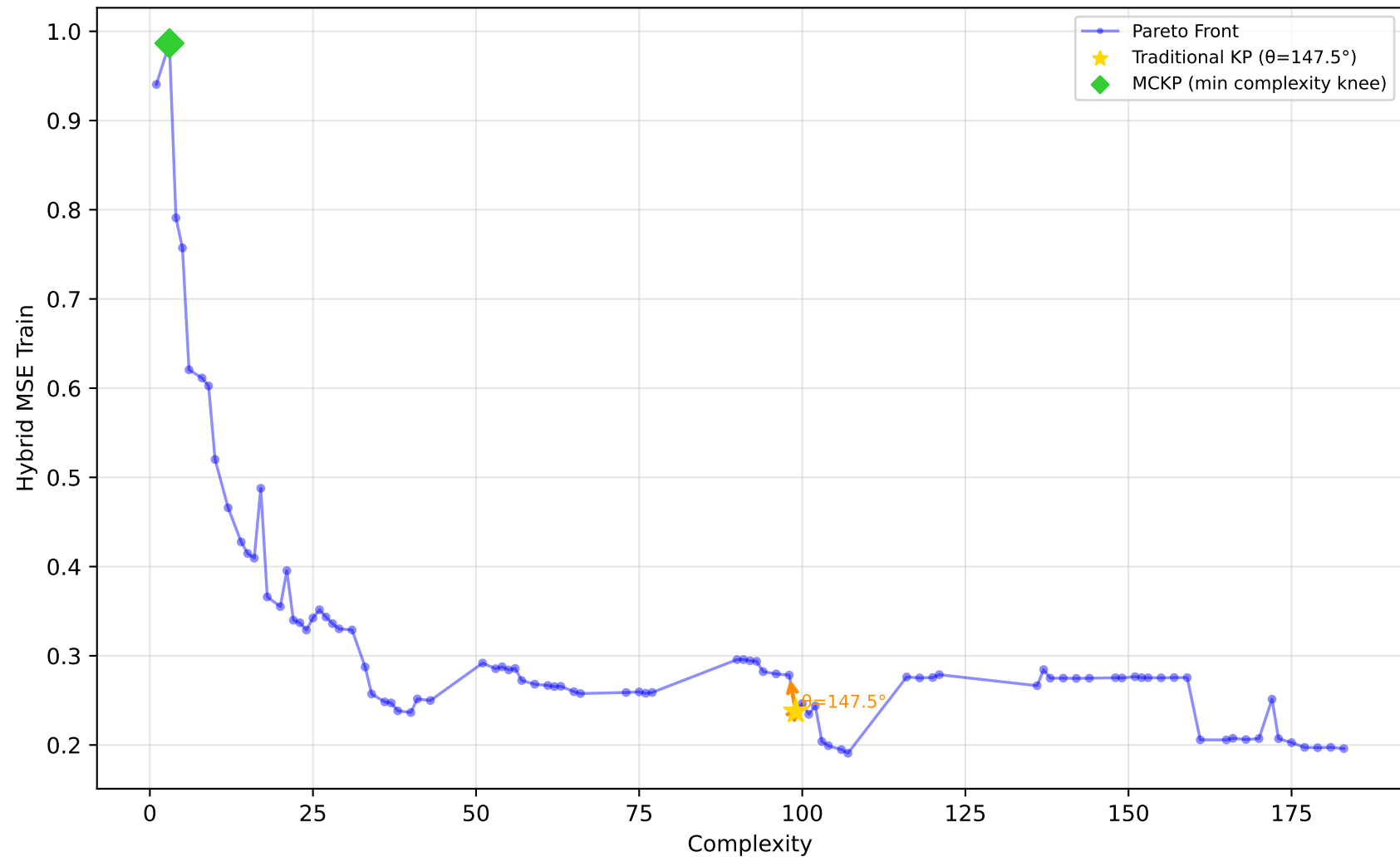
542_pollution - Run 20 - MVP - Hybrid MSE Train \lambda_1=1.00, \lambda_2=0.10, \lambda_3=0.00 | Difficulty: 0.63 | Method: hmr
