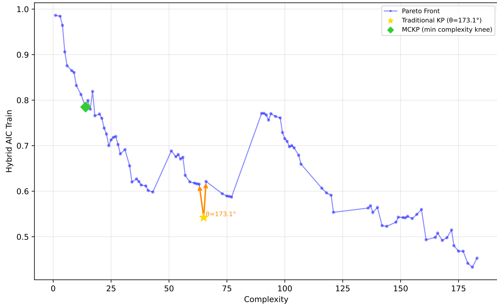
542_pollution - Run 20 - SVP - Hybrid AIC Train \lambda_1=0.00, \lambda_2=0.00, \lambda_3=0.20 | Difficulty: 0.63 | Method: hmr
