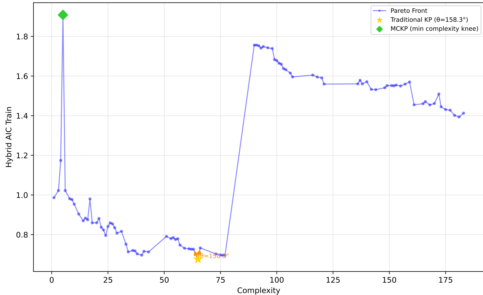
542_pollution - Run 20 - SVP - Hybrid AIC Train \lambda_1=0.70, \lambda_2=1.00, \lambda_3=0.10 | Difficulty: 0.63 | Method: hmr
