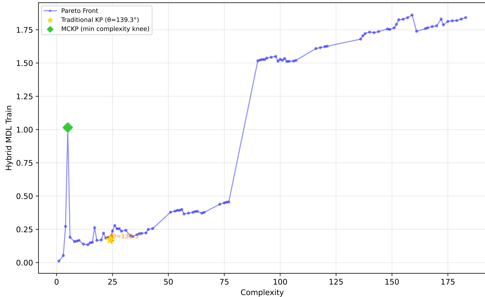
542_pollution - Run 20 - SVP - Hybrid MDL Train \lambda_1=0.70 , \bar{\lambda}_2=1.00 , \lambda_3=0.10 | Difficulty: 0.63 | Method: hmr
