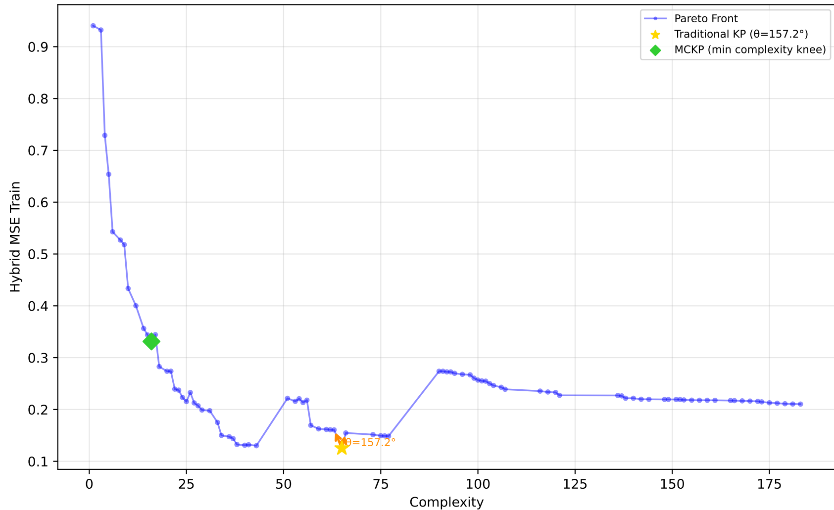
542_pollution - Run 20 - SVP - Hybrid MSE Train \lambda_1=0.00, \lambda_2=0.00, \lambda_3=0.20 | Difficulty: 0.63 | Method: hmr
