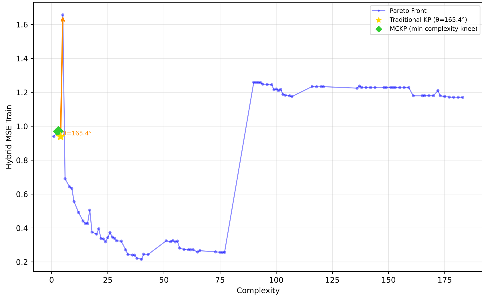
542_pollution - Run 20 - SVP - Hybrid MSE Train \lambda_1=0.70 , \lambda_2=1.00 , \lambda_3=0.10 | Difficulty: 0.63 | Method: hmr
