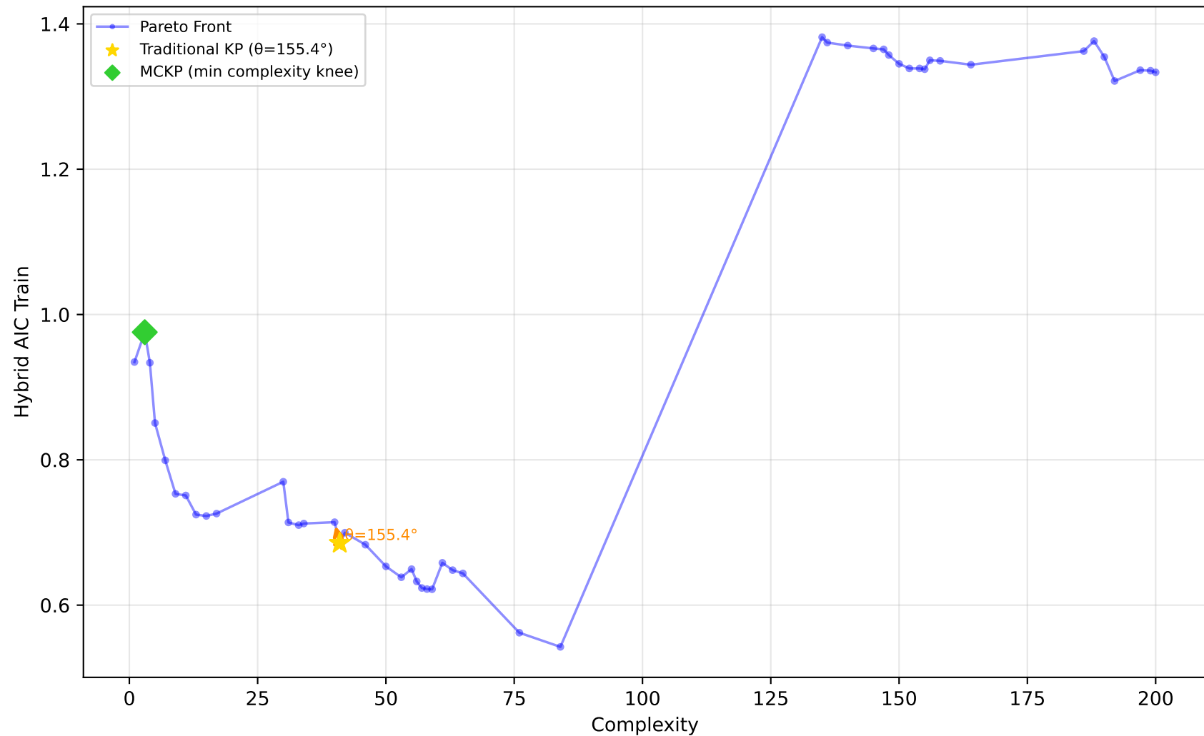
542_pollution - Run 21 - MVP - Hybrid AIC Train \lambda_1=1.00, \lambda_2=0.10, \lambda_3=0.00 | Difficulty: 1.00 | Method: hmr
