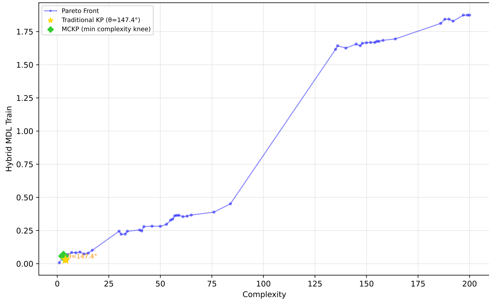
542_pollution - Run 21 - MVP - Hybrid MDL Train \lambda_1=1.00, \bar{\lambda}_2=0.10, \lambda_3=0.00 | Difficulty: 1.00 | Method: hmr
