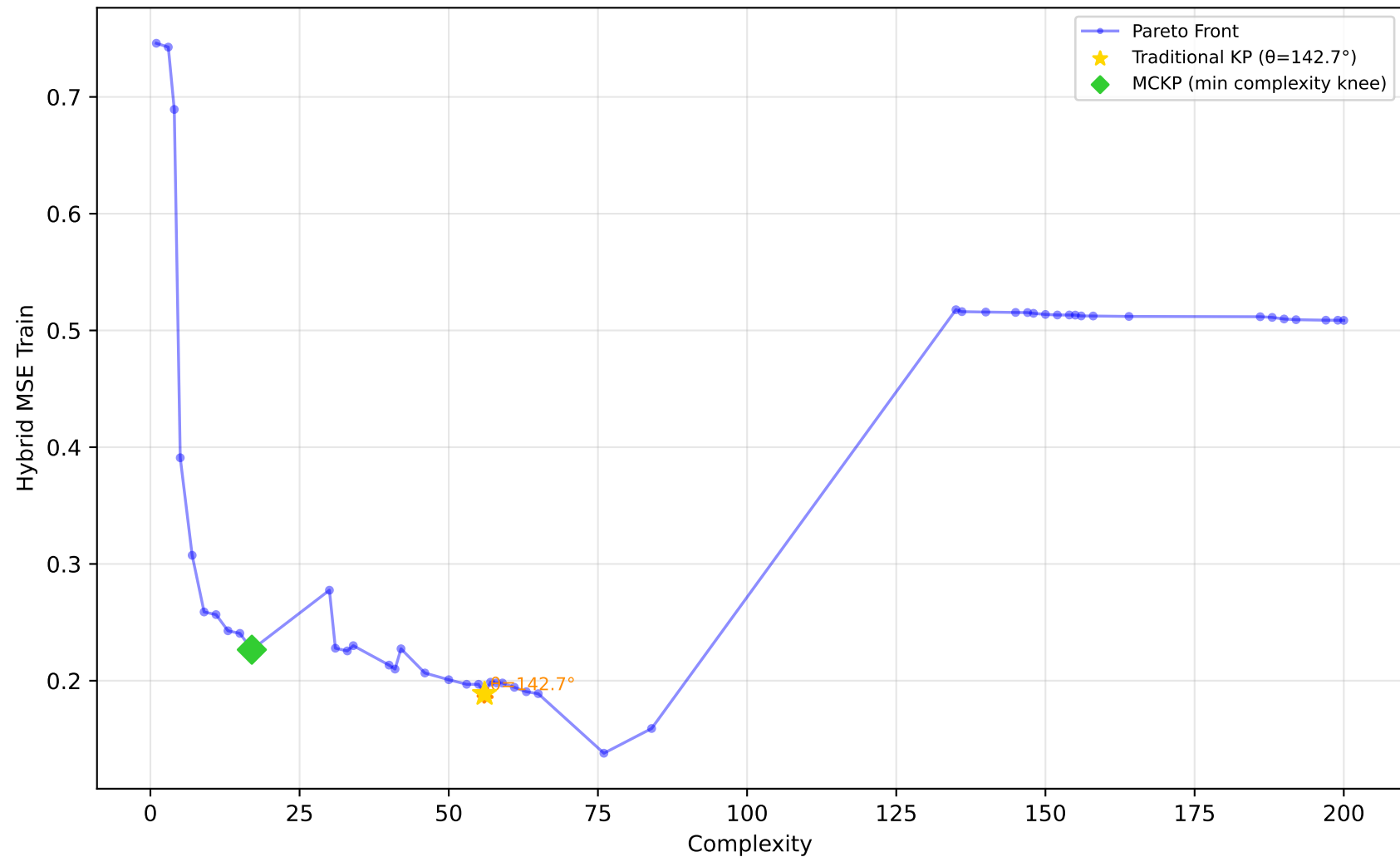
542_pollution - Run 21 - MVP - Hybrid MSE Train \lambda_1=0.40, \lambda_2=0.10, \lambda_3=0.00 | Difficulty: 1.00 | Method: hmr
