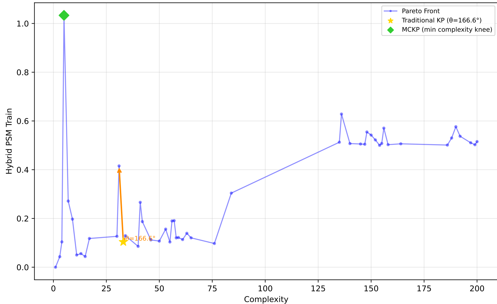
542_pollution - Run 21 - MVP - Hybrid PSM Train \lambda_1=0.40, \lambda_2=0.10, \lambda_3=0.00 | Difficulty: 1.00 | Method: hmr
