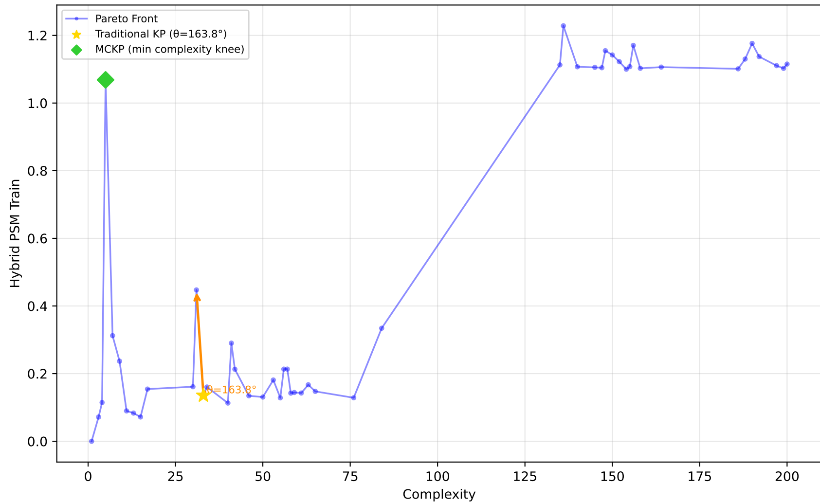
542_pollution - Run 21 - MVP - Hybrid PSM Train \lambda_1=1.00, \lambda_2=0.10, \lambda_3=0.00 | Difficulty: 1.00 | Method: hmr
