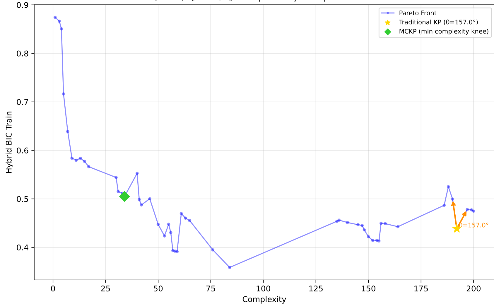
542_pollution - Run 21 - SVP - Hybrid BIC Train \lambda_1=0.00, \lambda_2=0.00, \lambda_3=0.20 | Difficulty: 1.00 | Method: hmr
