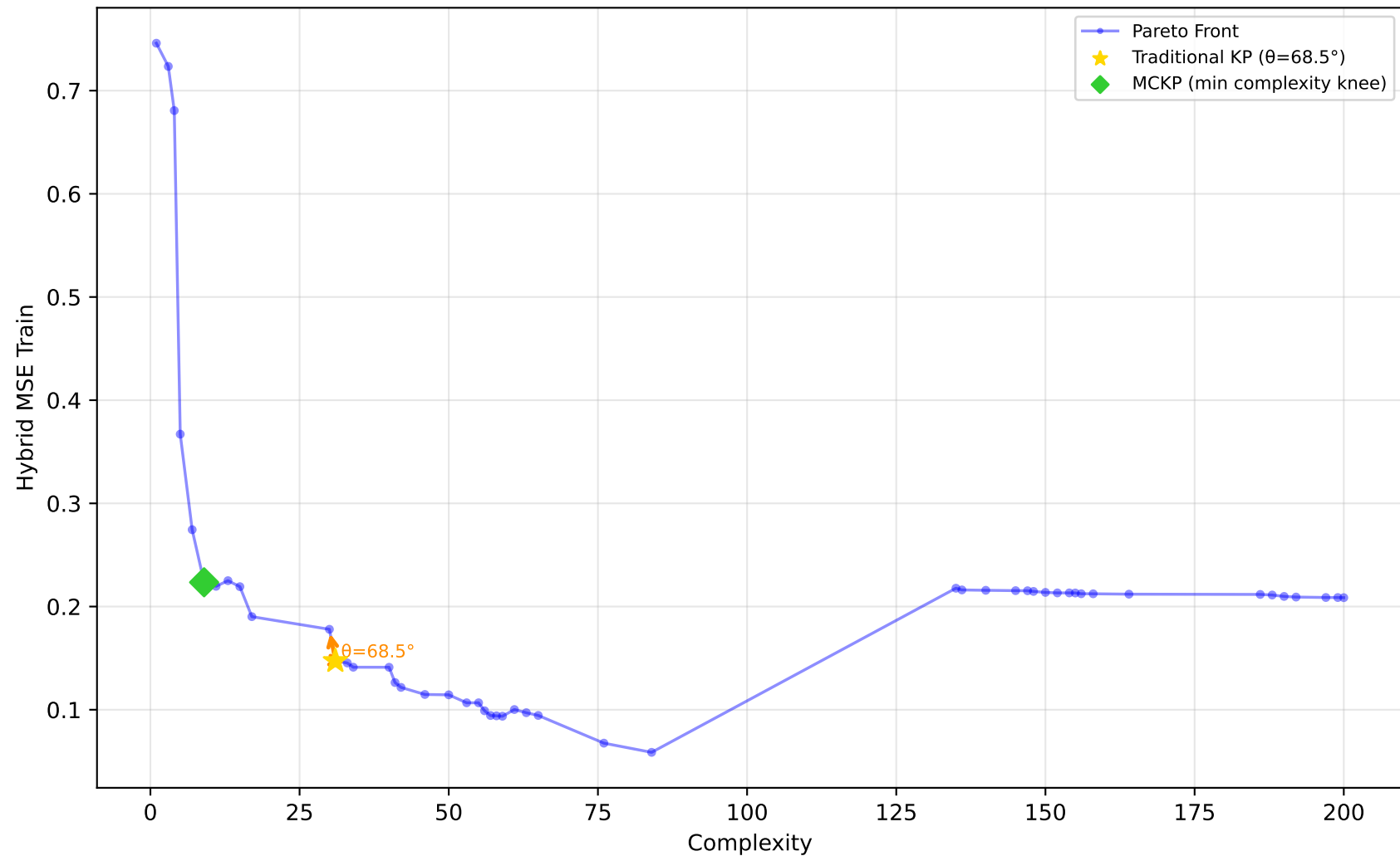
542_pollution - Run 21 - SVP - Hybrid MSE Train \lambda_1=0.00, \lambda_2=0.00, \lambda_3=0.20 | Difficulty: 1.00 | Method: hmr
