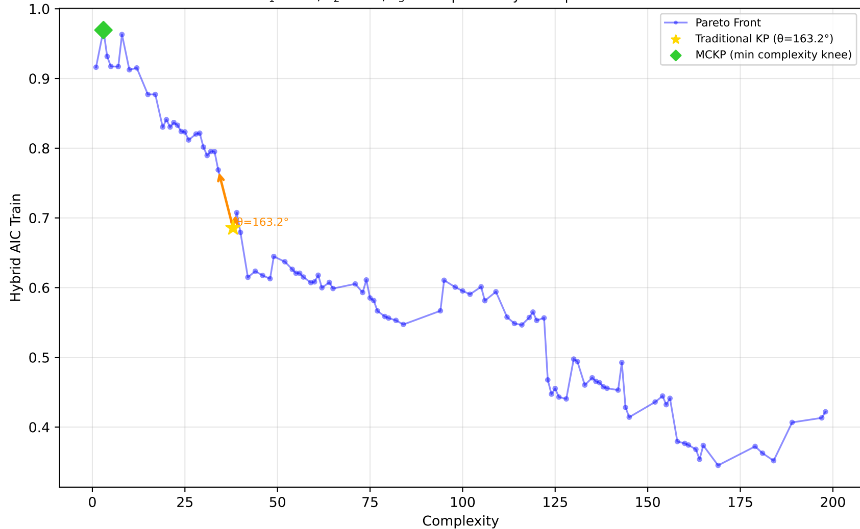
542_pollution - Run 22 - MVP - Hybrid AIC Train \lambda_1=1.00, \lambda_2=0.10, \lambda_3=0.00 | Difficulty: 1.00 | Method: hmr
