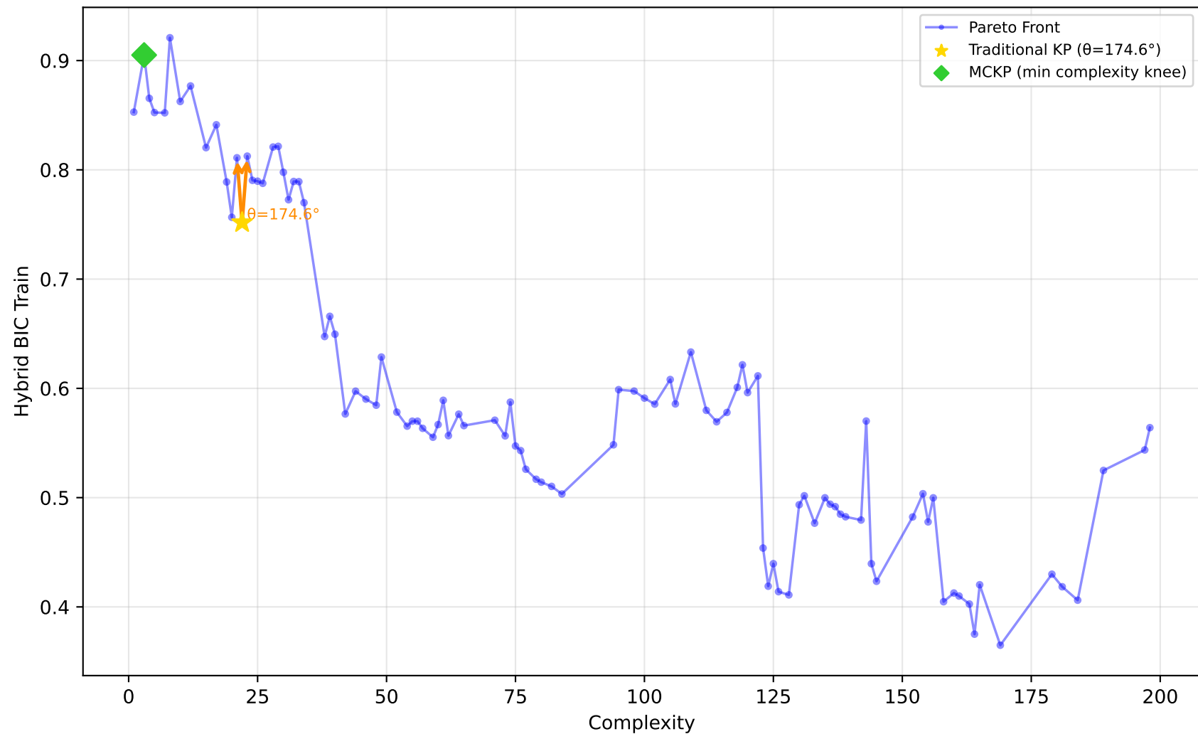
542_pollution - Run 22 - MVP - Hybrid BIC Train \lambda_1=1.00, \lambda_2=0.10, \lambda_3=0.00 | Difficulty: 1.00 | Method: hmr
