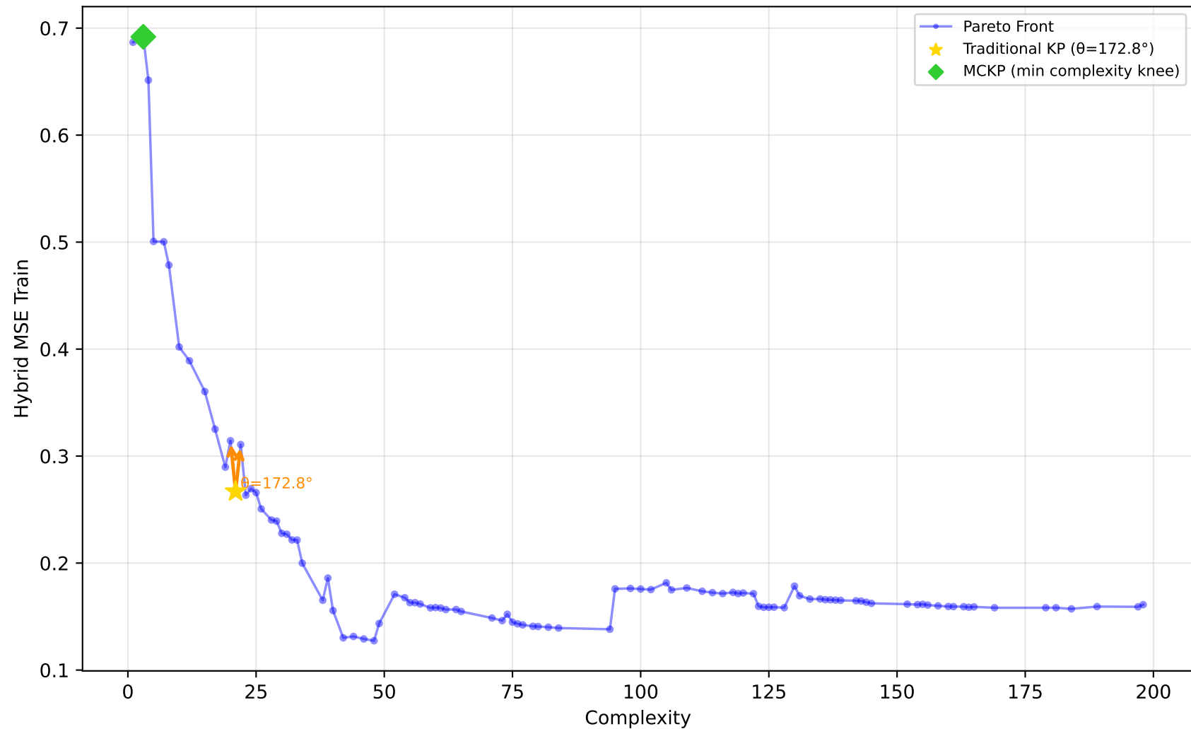
542_pollution - Run 22 - MVP - Hybrid MSE Train \lambda_1=0.40, \lambda_2=0.10, \lambda_3=0.00 | Difficulty: 1.00 | Method: hmr
