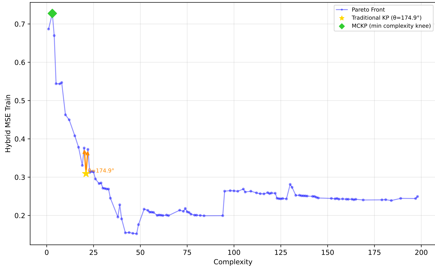
542_pollution - Run 22 - MVP - Hybrid MSE Train \lambda_1=1.00, \lambda_2=0.10, \lambda_3=0.00 | Difficulty: 1.00 | Method: hmr
