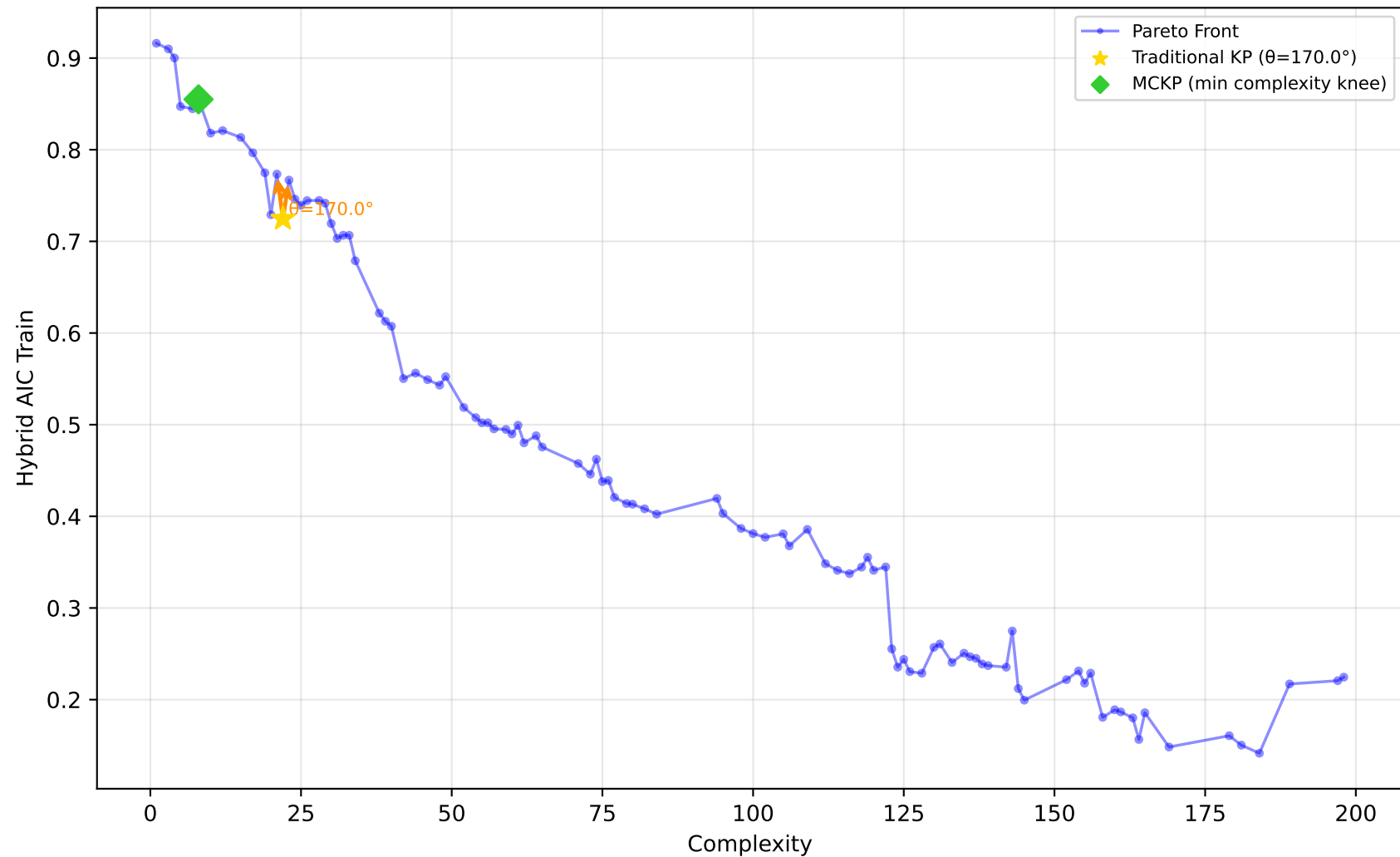
542_pollution - Run 22 - SVP - Hybrid AIC Train \lambda_1=0.00, \lambda_2=0.00, \lambda_3=0.20 | Difficulty: 1.00 | Method: hmr
