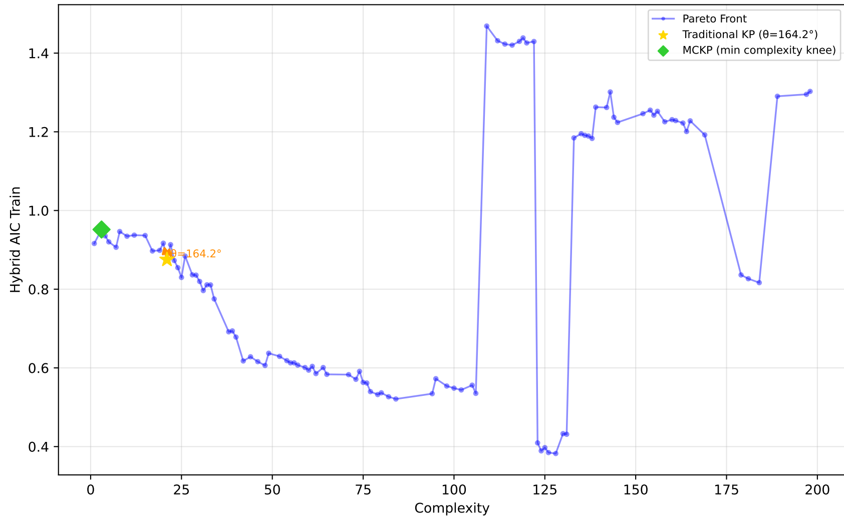
542_pollution - Run 22 - SVP - Hybrid AIC Train \lambda_1=0.70, \lambda_2=1.00, \lambda_3=0.10 | Difficulty: 1.00 | Method: hmr
