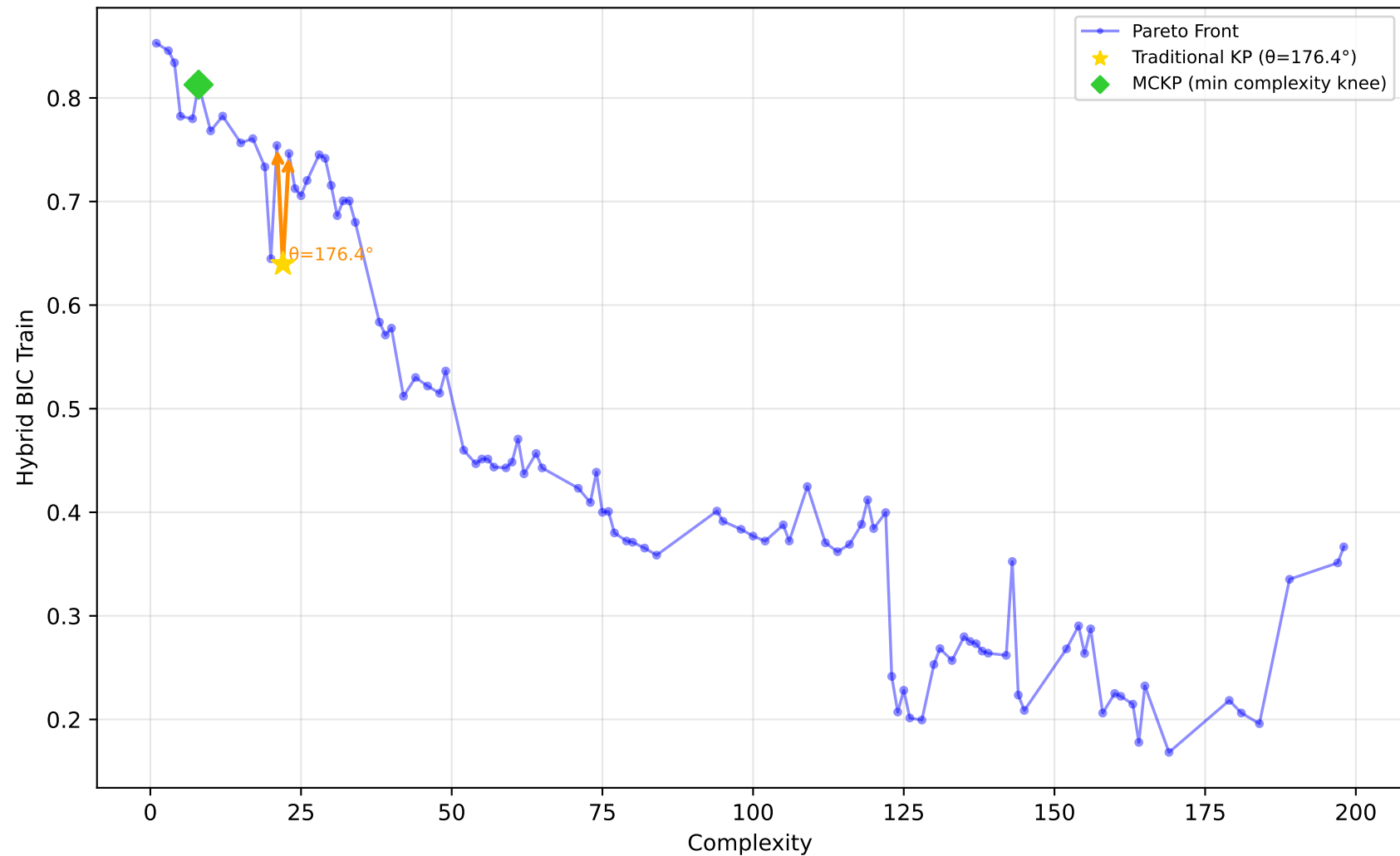
542_pollution - Run 22 - SVP - Hybrid BIC Train \lambda_1=0.00, \lambda_2=0.00, \lambda_3=0.20 | Difficulty: 1.00 | Method: hmr
