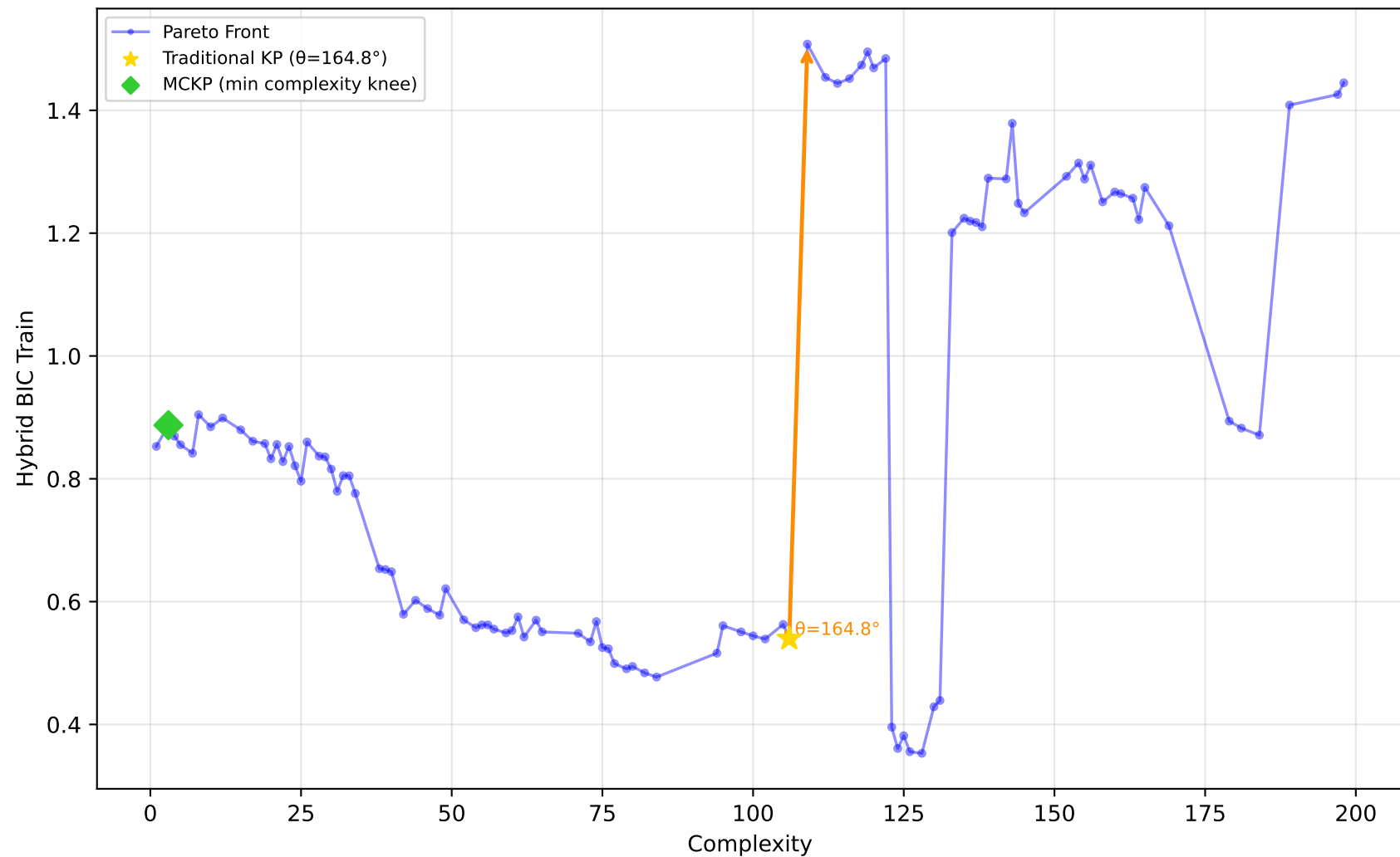
542_pollution - Run 22 - SVP - Hybrid BIC Train \lambda_1=0.70, \lambda_2=1.00, \lambda_3=0.10 | Difficulty: 1.00 | Method: hmr
