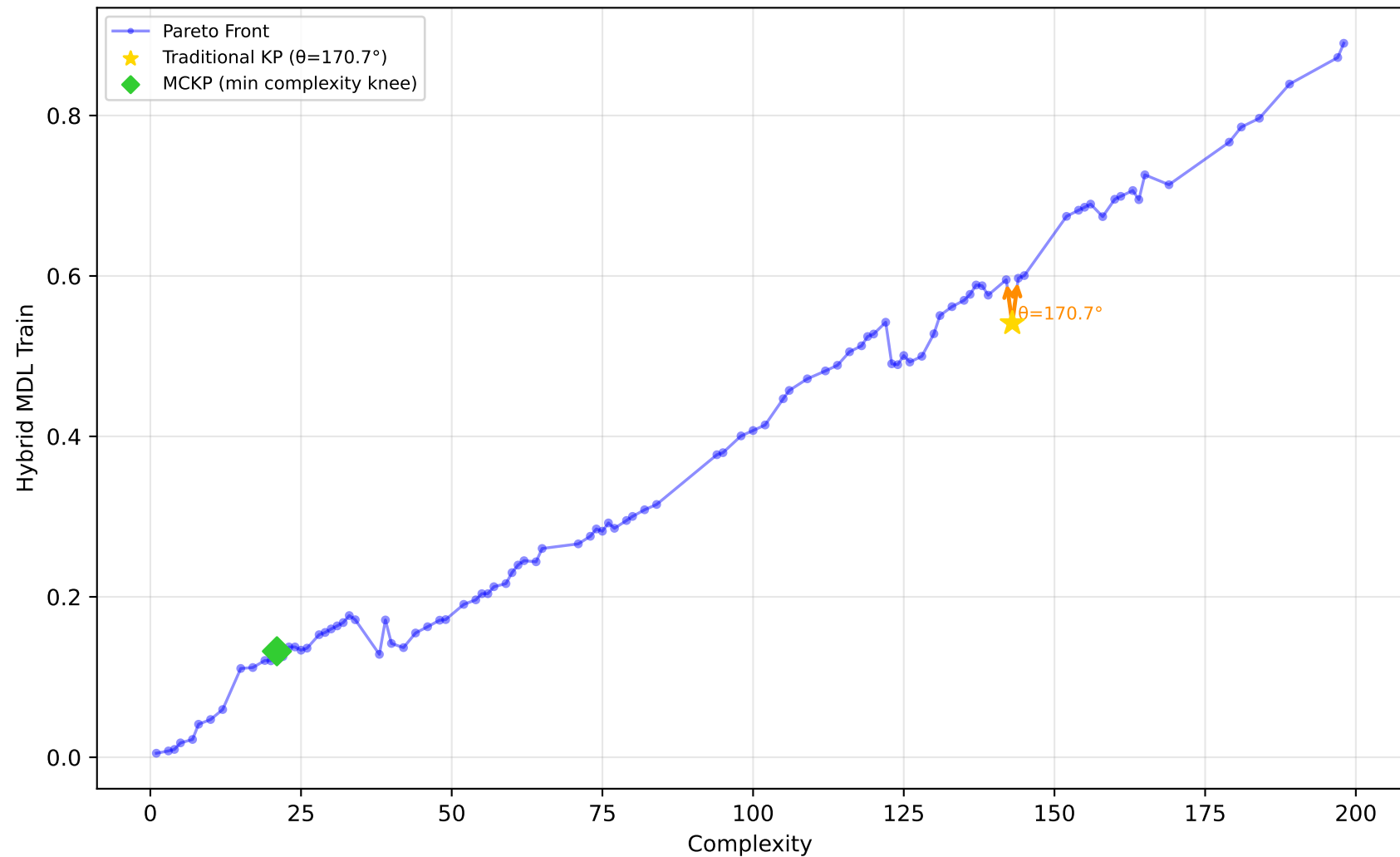
542_pollution - Run 22 - SVP - Hybrid MDL Train \lambda_1=0.00, \lambda_2=0.00, \lambda_3=0.20 | Difficulty: 1.00 | Method: hmr
