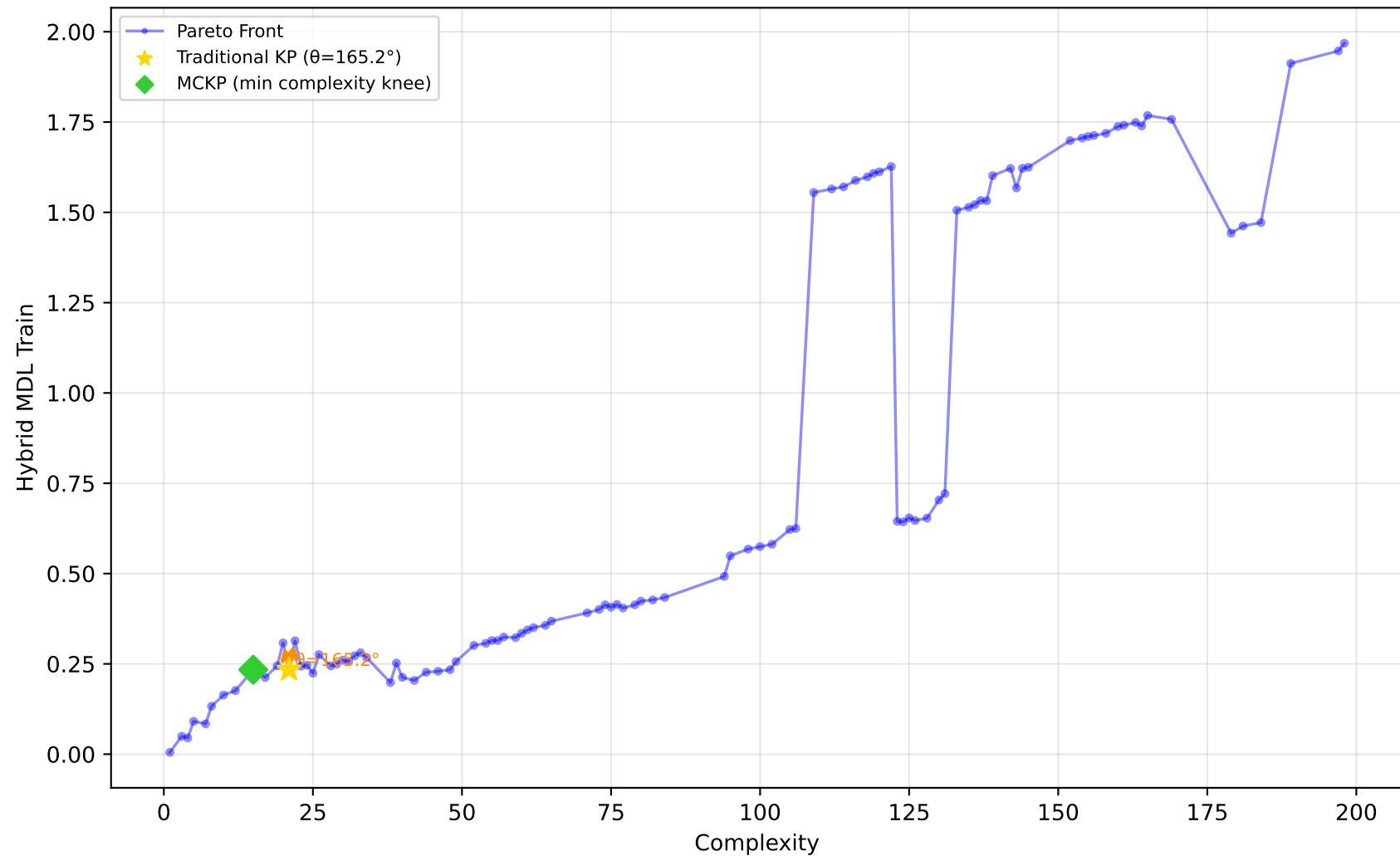
542_pollution - Run 22 - SVP - Hybrid MDL Train \lambda_1=0.70 , \bar{\lambda}_2=1.00 , \lambda_3=0.10 | Difficulty: 1.00 | Method: hmr
