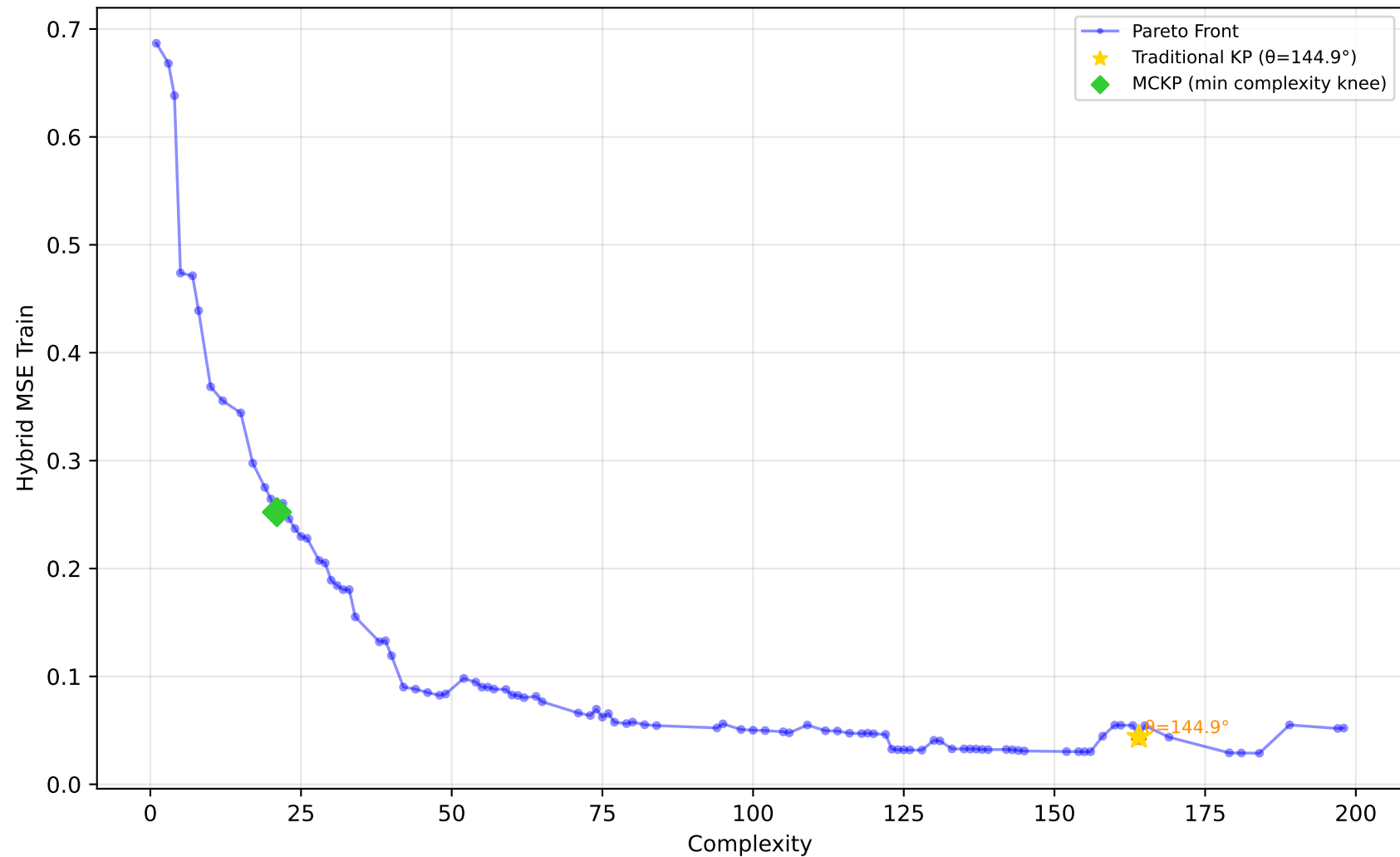
542_pollution - Run 22 - SVP - Hybrid MSE Train \lambda_1=0.00, \lambda_2=0.00, \lambda_3=0.20 | Difficulty: 1.00 | Method: hmr
