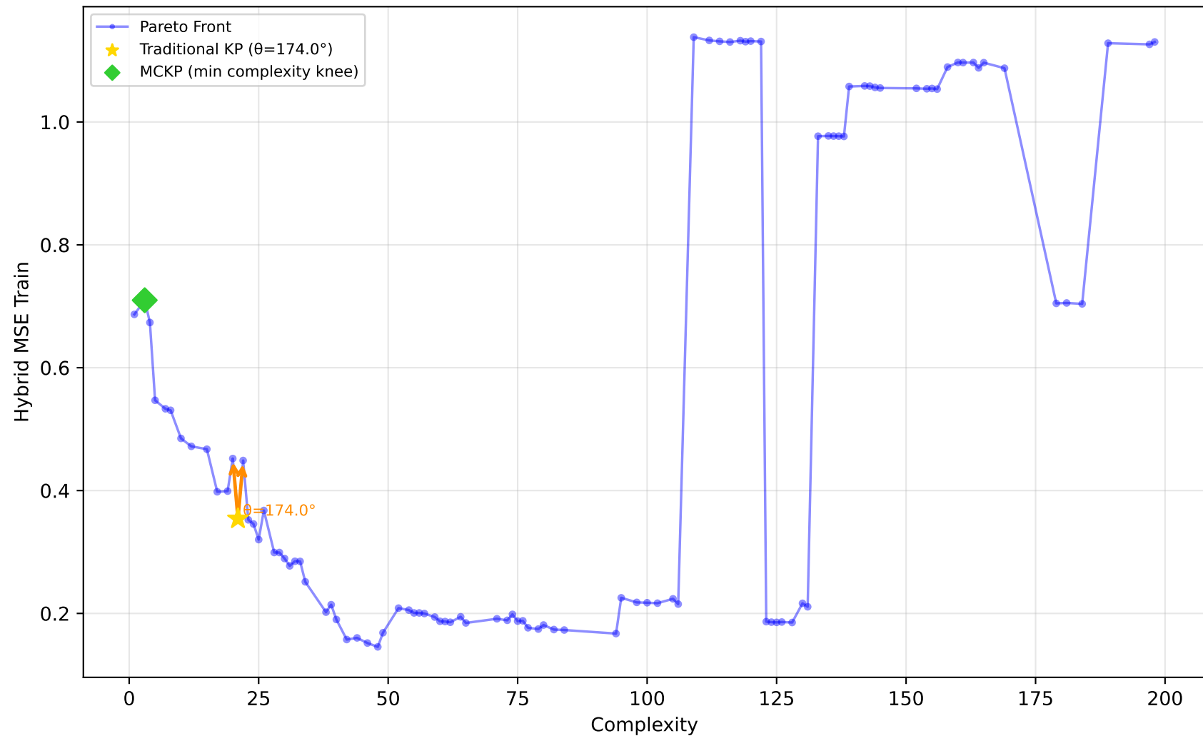
542_pollution - Run 22 - SVP - Hybrid MSE Train \lambda_1=0.70, \lambda_2=1.00, \lambda_3=0.10 | Difficulty: 1.00 | Method: hmr
