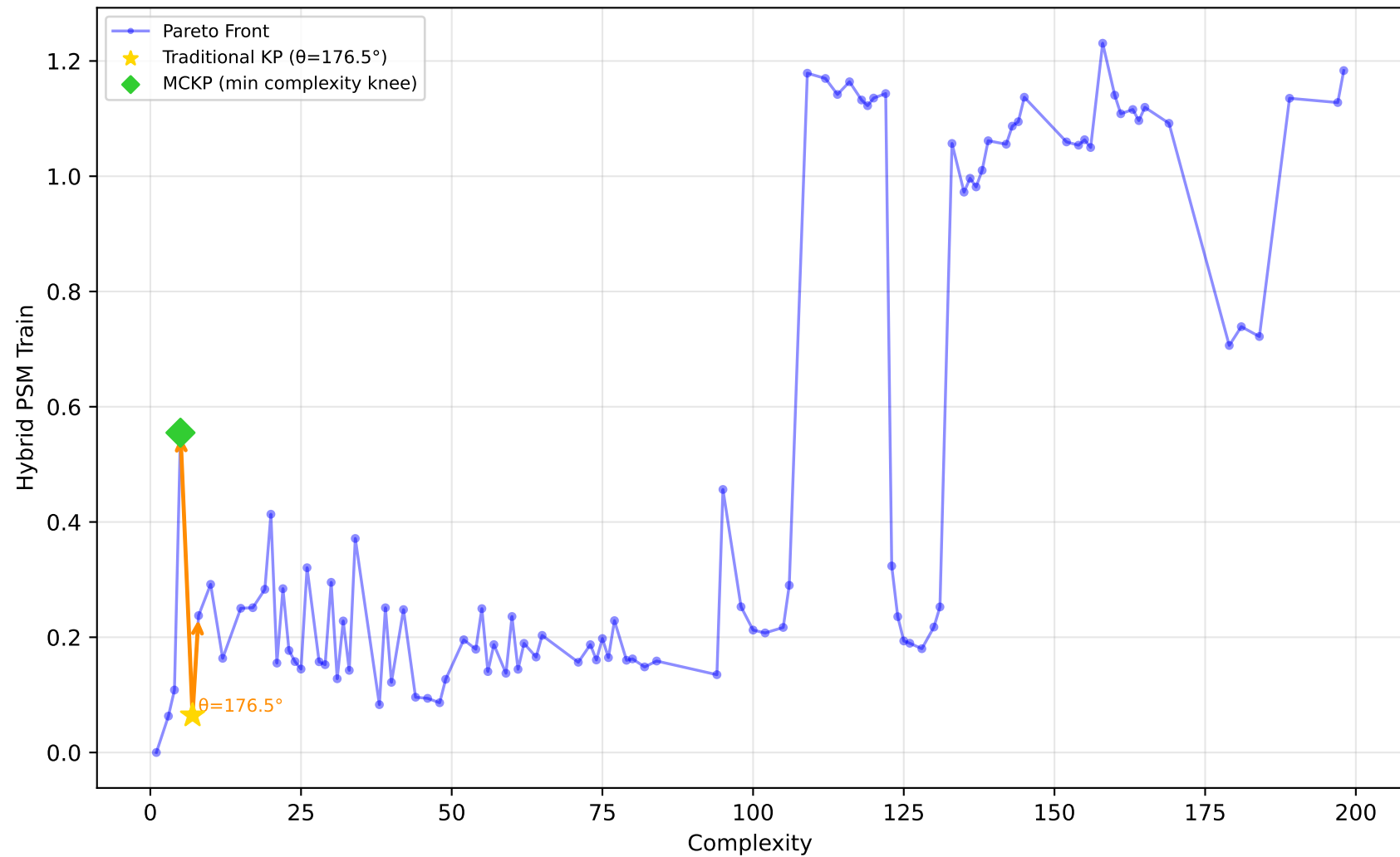
542_pollution - Run 22 - SVP - Hybrid PSM Train \lambda_1=0.70, \lambda_2=1.00, \lambda_3=0.10 | Difficulty: 1.00 | Method: hmr
