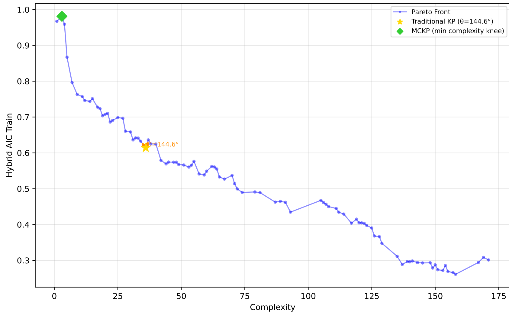
542_pollution - Run 23 - MVP - Hybrid AIC Train \lambda_1=0.40, \lambda_2=0.10, \lambda_3=0.00 | Difficulty: 0.25 | Method: mckp
