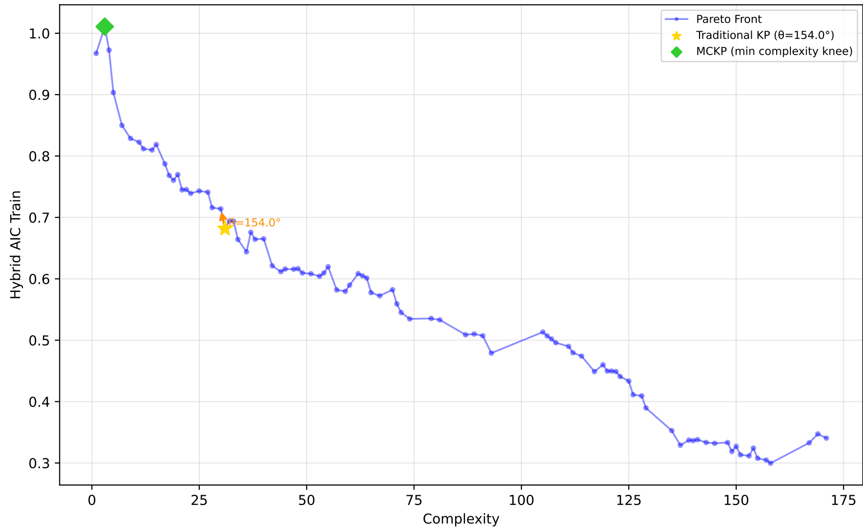
542_pollution - Run 23 - MVP - Hybrid AIC Train \lambda_1=1.00, \lambda_2=0.10, \lambda_3=0.00 | Difficulty: 0.25 | Method: mckp
