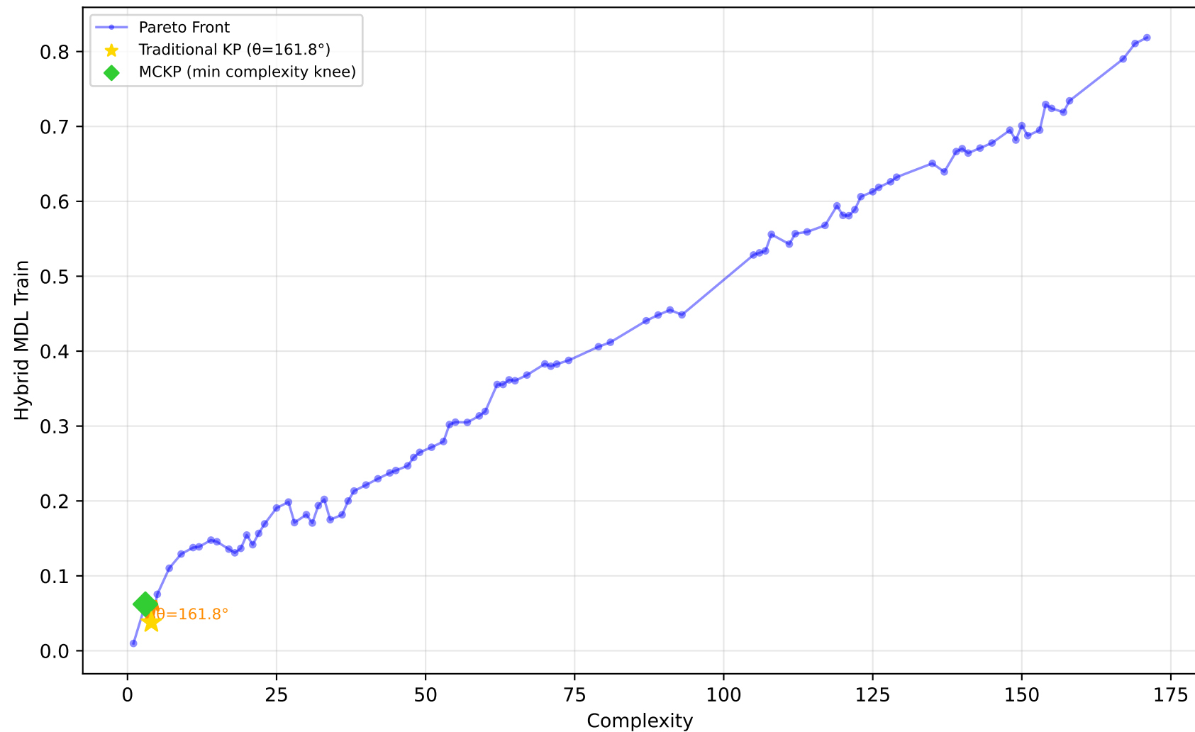
542_pollution - Run 23 - MVP - Hybrid MDL Train \lambda_1=1.00, \lambda_2=0.10, \lambda_3=0.00 | Difficulty: 0.25 | Method: mckp
