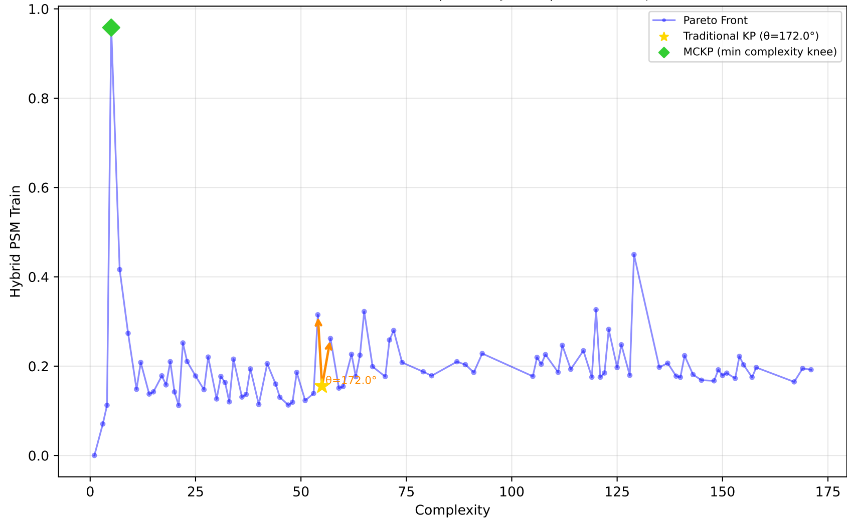
542_pollution - Run 23 - MVP - Hybrid PSM Train \lambda_1=1.00, \bar{\lambda}_2=0.10, \lambda_3=0.00 | Difficulty: 0.25 | Method: mckp
