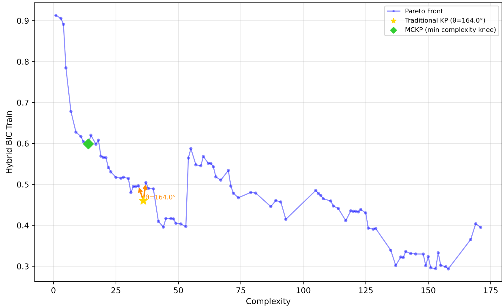
542_pollution - Run 23 - SVP - Hybrid BIC Train \lambda_1=0.00, \lambda_2=0.00, \lambda_3=0.20 | Difficulty: 0.25 | Method: mckp
