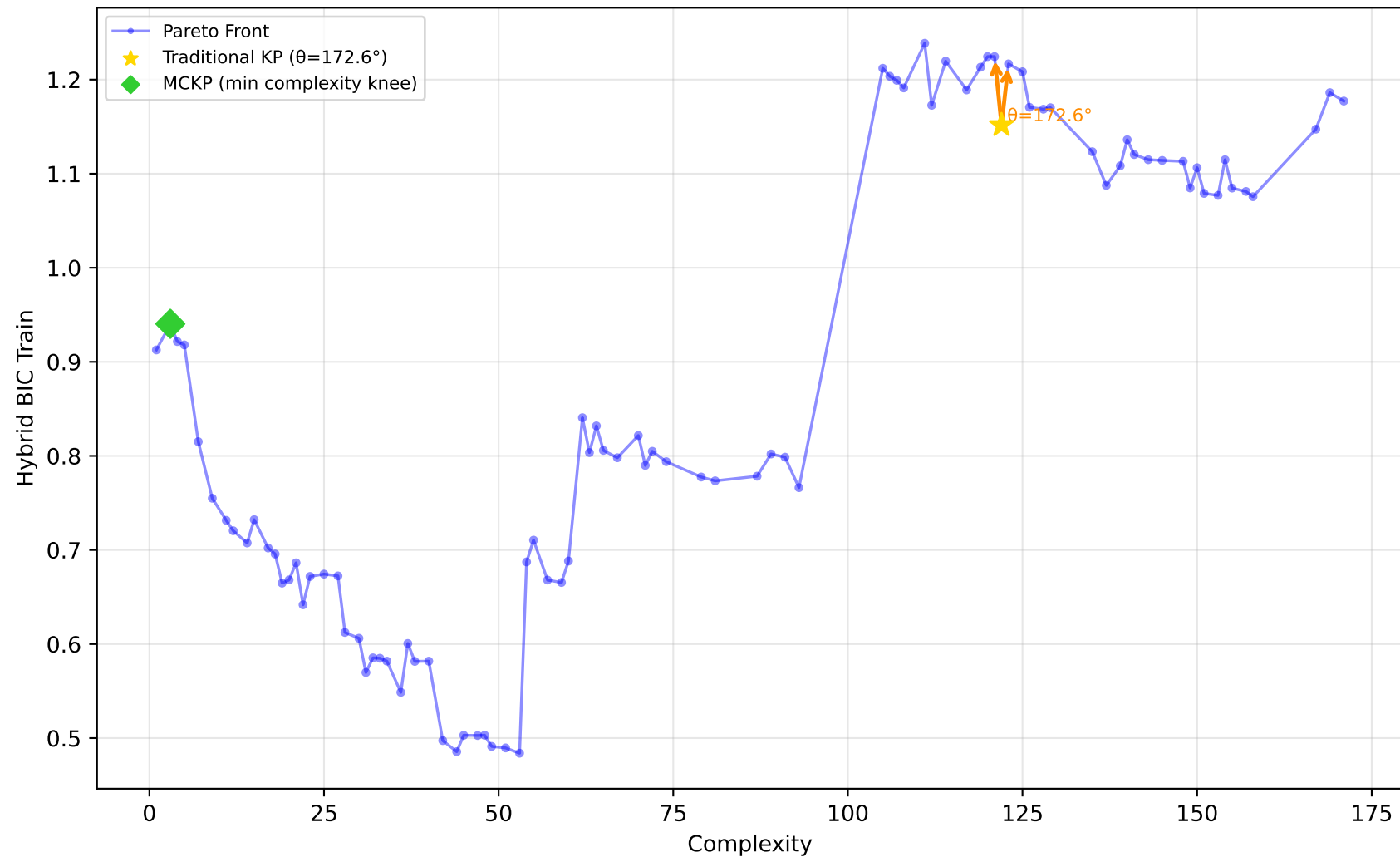
542_pollution - Run 23 - SVP - Hybrid BIC Train \lambda_1=0.70, \lambda_2=1.00, \lambda_3=0.10 | Difficulty: 0.25 | Method: mckp
