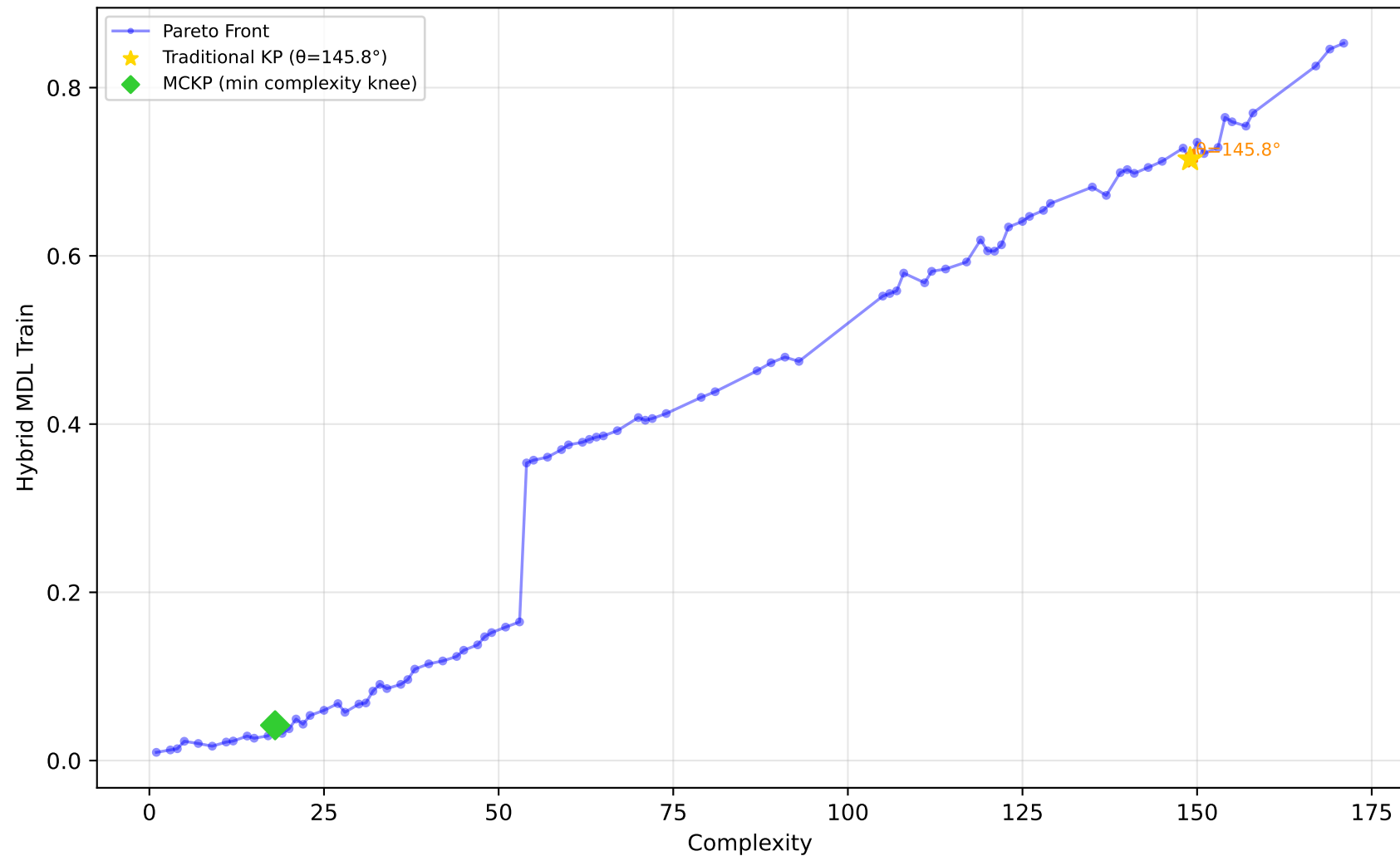
542_pollution - Run 23 - SVP - Hybrid MDL Train \lambda_1=0.00, \lambda_2=0.00, \lambda_3=0.20 | Difficulty: 0.25 | Method: mckp
