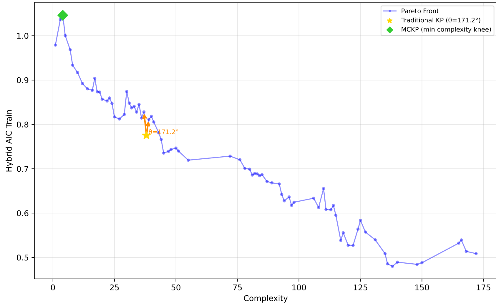
542_pollution - Run 24 - MVP - Hybrid AIC Train \lambda_1=1.00, \lambda_2=0.10, \lambda_3=0.00 | Difficulty: 0.39 | Method: mckp
