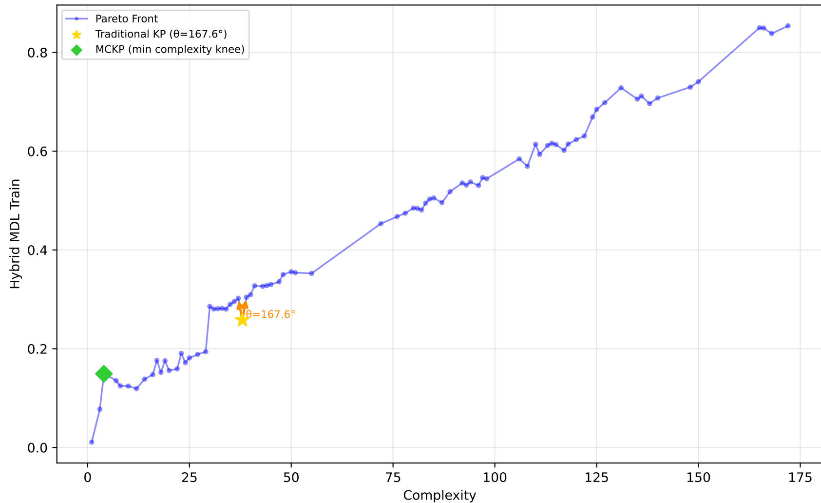
542_pollution - Run 24 - MVP - Hybrid MDL Train \lambda_1=1.00, \lambda_2=0.10, \lambda_3=0.00 | Difficulty: 0.39 | Method: mckp
