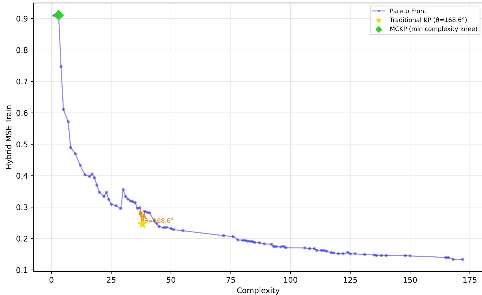
542_pollution - Run 24 - MVP - Hybrid MSE Train \lambda_1=0.40, \lambda_2=0.10, \lambda_3=0.00 | Difficulty: 0.39 | Method: mckp
